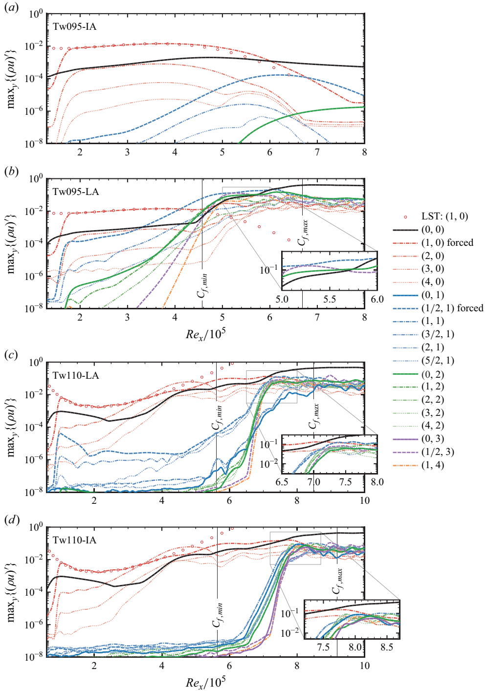
Figure 11. Streamwise evolution of the y-maximum of (\rho u)' for the most relevant modes (\omega/\omega_{2-D}, \beta/\beta_0) for cases (a) Tw095-IA, (b) Tw095-LA, (c) Tw110-LA, and (d) Tw110-IA. The minimum and maximum values of the time- and spanwise-averaged skin-friction coefficient are indicated as C_{f,min} = \min\{C_f\} and C_{f,max} = \max\{C_f\} , respectively. Insets in (c) and (d) highlight the relevant modes in the breakdown region. Note the different Re_x -axis limits between the subcritical (a,b) and (c,d) transcritical cases.
