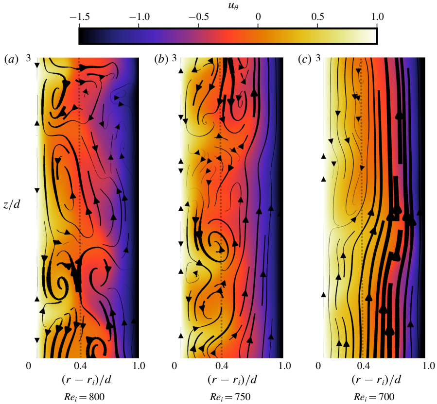
FIGURE 3. Streamlines overlay snapshots of the azimuthal velocity u_\theta in the meridional plane for Re_o = -1200 . The thickness of the streamlines represents the norm of the velocity vector (u_r, u_z) . We observe chaotic motion for all r in the ‘featureless turbulent’ flow (a). With decreasing Re_i , laminarization occurs from the outer cylinder towards the inner cylinder (b,c). The vertical dashed lines at (r - r_i)/d \approx 0.4 give the location of the nodal plane of neutral stability. The meridional snapshots were obtained at \theta = \pi .
