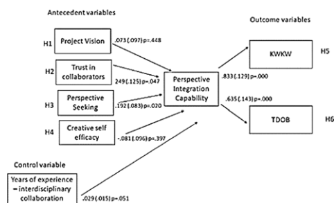
Figure 1. Study 5 Structural equation model.
