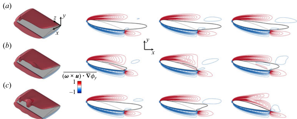
Figure 13. Lift elements around an untapered unswept wing ( \lambda, \Lambda = 1, 0^\circ ) at \alpha = 14^\circ , (a) baseline, (b) controlled flows with St = 0.14 and (c) St = 0.18 forcing modes. Leftmost figures show 3-D time-averaged lift elements with isosurfaces of (\omega \times \mathbf{u}) \cdot \nabla \phi_y = \pm 1 . To the right of the 3-D view, slices at z/c = 0.5, 0.8 and 1.2 show the red and blue contours of lift elements and a black line contour of \overline{u_x} = 0 .
