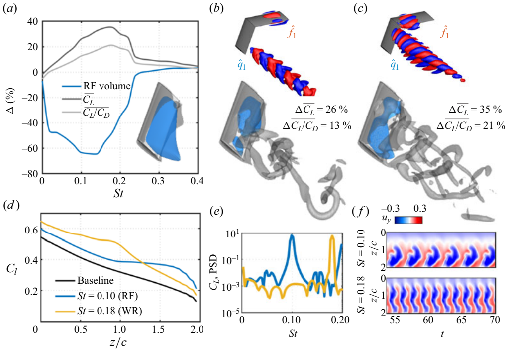
Figure 14. Assessment of flow modification using forcing-mode actuation for an untapered swept wing ( \lambda, \Lambda = 1, 30^\circ ). Control with forcing modes located over the reversed-flow (RF) bubble and wing root (WR) are covered in detail. (a) Reversed-flow volume contraction and aerodynamic changes for controlled flows. Baseline flow on the bottom-right corner. (b,c) On top, isosurfaces of forcing \hat{f}_{uy} = \pm 1 and response modes \hat{q}_{uy} = \pm 0.5 at (b) St = 0.10 and (c) St = 0.18 . On the bottom, instantaneous controlled flows over half-span. All flows are visualized with grey-coloured isosurfaces of Q = 1 and blue-coloured isosurfaces of \overline{u_x} = 0 . (d) Plot of C_l versus wingspan, (e) lift PSD and (f) probed u_y for controlled flows.
