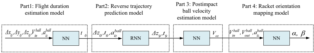
Figure 10. Proposed cascade neural network.
