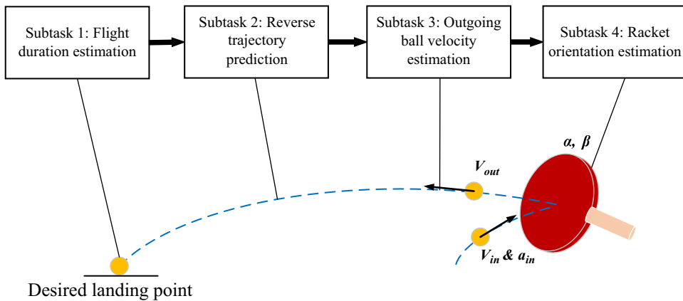
Figure 9. Planning of ball landing position control subtasks.
