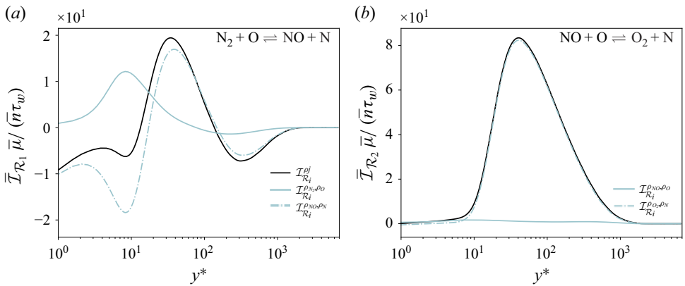
Figure 22. Fine-grained decomposition of turbulence–chemistry interaction induced by partial-density fluctuations for the Zel’dovich exchange reactions (a) (R1) and (b) (R2).
