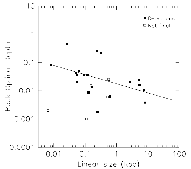
Figure 2 Peak optical depth versus linear size. Filled squares represent HI absorption detections, while open squares are preliminary detections. A clear correlation is found with a probability >95\% , which is enough to explain the correlation in Figure 1.
