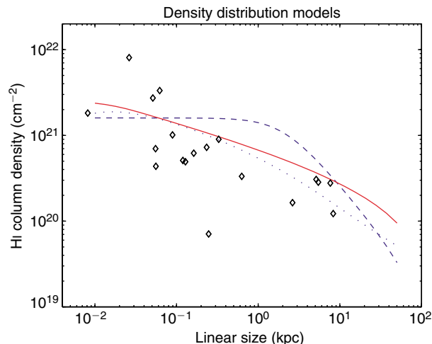
Figure 3 Results of calculating the expected HI column density given different density profiles. The diamonds represent the real data. The spherical King density profile, plotted with a dashed line, cannot reproduce the observed HI column density distribution for any value of \beta . Instead, a power law drop of the density provides a more similar distribution, with the closest fit for \beta = 1.25 and n_0 = 2.7 \times 10^{-2} \text{ cm}^{-3} (solid line). The dotted line represents a disk distribution; it is possible to find reasonable fits for a large range of opening angles.
