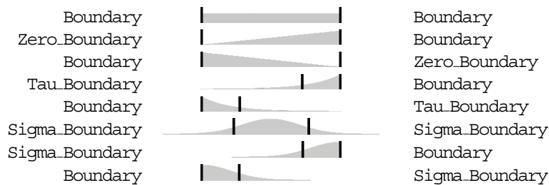
Figure 4 Range of grouping distributions supported in OxCal v4.0. Groupings are defined by using Boundary commands within a Sequence . All events sandwiched between 2 boundaries (including those in nested phases) are treated as a single group. The type of group is defined by the type of boundary used. A simple Boundary at the start and end of a group defines a uniform phase. A Zero_Boundary is used to define the start or end of a group where the event rate has a ramped distribution. A Tau_Boundary can be used to define an exponentially distributed group and a pair of Sigma_Boundary statements, a normal distribution. The latter two types of group allow the events to spill beyond the dates of the boundaries themselves and allow the creation of models of processes that do not have definite start and end events.
