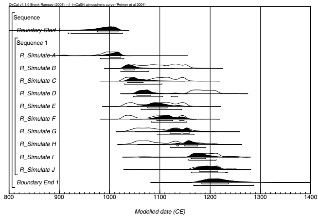
Figure 8 This figure shows two kinds of simulation that can be useful. At the top, we have a simulation of a sequence of 10 events assumed to be from the period 1000–1200 CE. In this simulation, we include no dating information but only the order of the events. On the left is the model definition in OxCal’s CQL and on the right the effect of the model prior on the dates within the sequence. Even without any dating information, a sequential prior does have a considerable effect on the intervening dates. Below this, there is a simulation of a series of 10 14 C dates, assumed to come from the same period. The plot on the right shows the kind of resolution one might expect to get from such a model, in this period, with uncertainty terms on the 14 C dates of ±25. Comparison of this plot with the one above shows the degree to which the 14 C dates and the model define the final posterior distributions.
