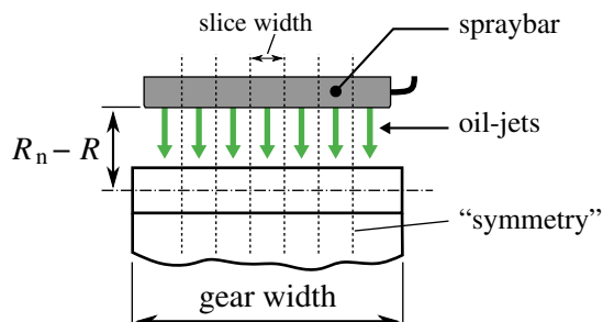
Figure 2. Illustration of the investigated slice of a gear and the nozzle position.
