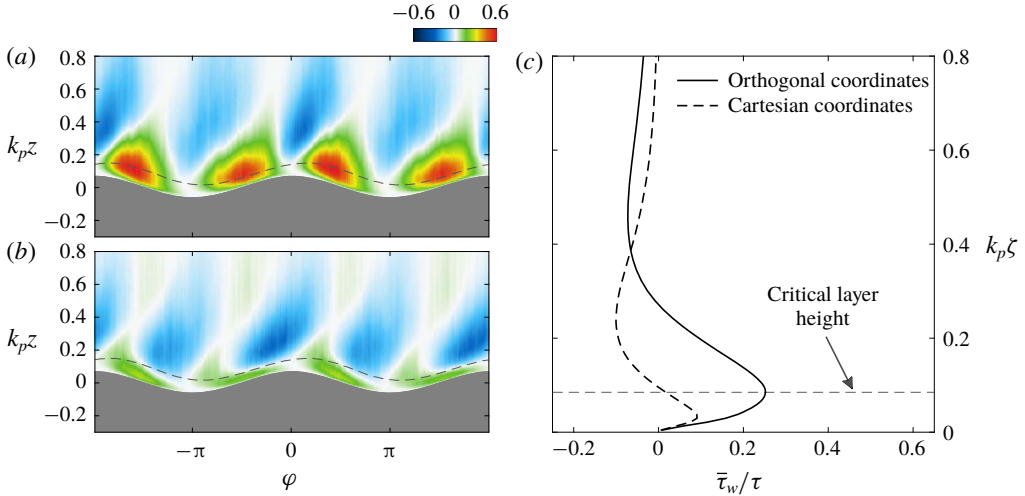
FIGURE 13. Phase-averaged distribution of the wave-induced stress normalized by the total stress, i.e. \langle \tau_w \rangle / \tau , calculated using (a) orthogonal curvilinear coordinates \tau_w = -\rho \tilde{U}_1 \tilde{U}_3 and (b) Cartesian coordinates \tau_w = -\rho \tilde{u}_1 \tilde{u}_3 for the lowest wind speed of U_{10} = 2.25 \text{ m s}^{-1} . (c) The profiles of the normalized mean wave-induced stress \bar{\tau}_w/\tau . The phase-averaged and mean profile fields are plotted above the mean water surface as a function of the dimensionless distance k_p z and k_p \zeta , respectively. The grey dashed lines indicate the location of the critical layer.
