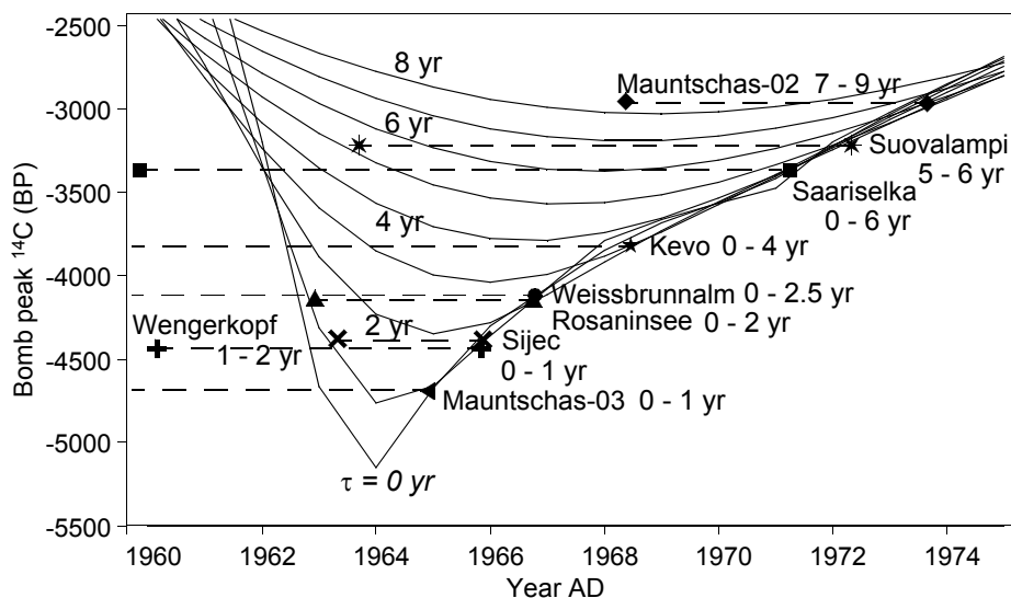
Figure 3 Illustration of the assessment of the integration time \tau . The smooth lines represent “theoretical” profiles of 14 C age, obtained for different values of integration time. The maximum 14 C values measured in particular profiles are represented by horizontal segments. The lengths of the segments correspond to the time intervals between adjacent samples in particular peat profiles.
