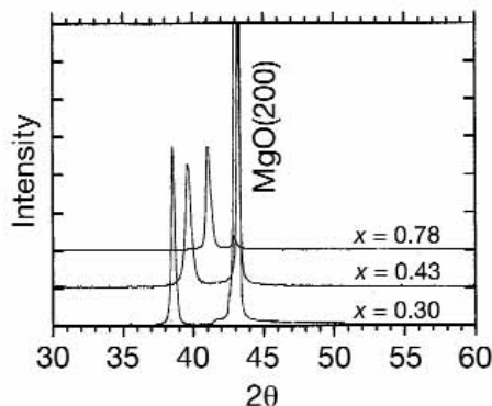
Figure 2. Diffraction patterns in the 30^\circ – 60^\circ range from \text{Ca}_{(1-x)}\text{Ni}_x\text{O} films fabricated from different Ca-Ni-K targets. The substrate is single-crystal MgO.
