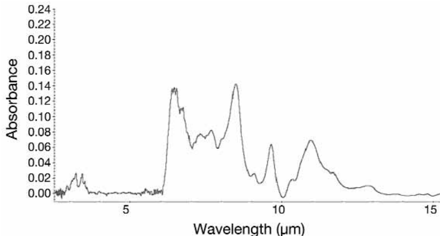
Figure 2. Fourier transform infrared spectrum of a polypyrrole film.
