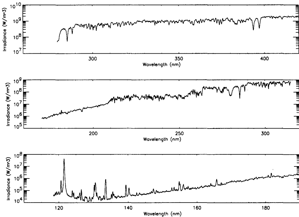
FIGURE 2. Bottom panel: Spectrum obtained from short wavelength channel of the SOLSTICE. Middle panel: Spectral data from middle wavelength channel. Top panel: Spectral data from the long wavelength channel.
