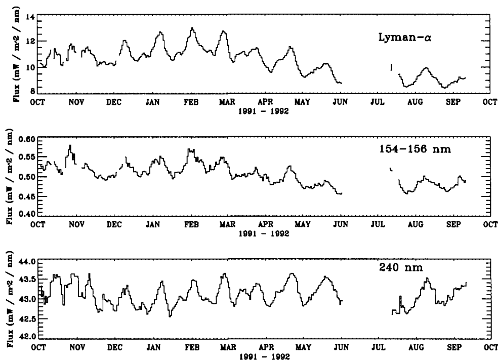
FIGURE 4. One year of SOLSTICE solar data at three separate wavelengths. (The enhanced tick marks denote the beginning of each month.)
