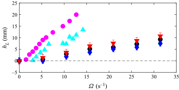
Figure 3. Levitation height h_L (mm) as a function of the rotational speed \Omega (s -1 ) for the Boger fluids (BF-I and BF-II). The symbols for the experiments correspond to those in table 1. The dashed line shows the measurements for the Newtonian case (no levitation observed).
