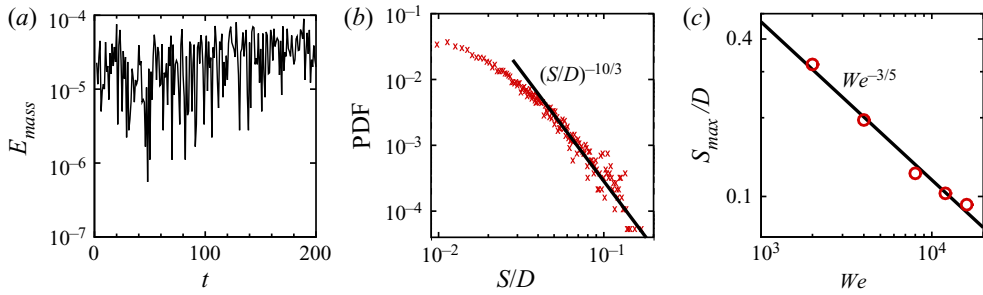
Figure 2. (a) Temporal evolution of mass error E_{mass} and (b) probability density function (PDF) of the drop size S/D at We = 16\,000 , where D is the domain height and S = 2\sqrt{A/\pi} with A being the drop area. (c) Maximal drop size S_{max}/D as function of We , where S_{max} is measured in the same way as in Hinze (1955), that is, the diameter of the equivalent drop occupying 95 % of the total dispersed area.
