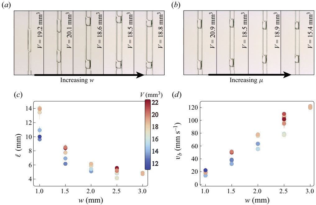
Figure 4. Bridge geometry. (a,b) Typical bridge profile for (a) increasing fibre gap w with fixed viscosity \mu , and (b) increasing viscosity \mu with fixed fibre gap w , both with r_f = 0.25 \text{ mm} . (c) Bridge length \ell and (d) velocity v_b against fibre gap w for bridge volume 11.5 \leq V \leq 22 \text{ mm}^3 , where the marker colour corresponds to the volume given in the colour bar. The fibre radius is r = 0.25 \text{ mm} , and liquid viscosity is \mu = 90 \text{ mPa} \cdot \text{s} . Bridge length decreases nonlinearly as w increases, while bridge velocity increases with w and increases with V .
