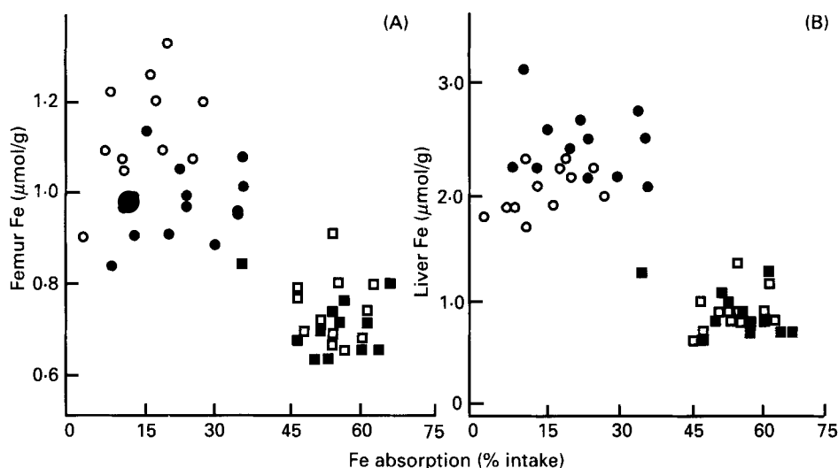
Fig. 2. Relationships between apparent iron absorption and either (A) femur Fe concentration ( r = 0.78 , n = 48 , P < 0.001 ) or (B) hepatic Fe concentration ( r = 0.81 , n = 48 , P < 0.001 ) for all individual animals of Expt 2. (○, □), Rats fed on an adequate amount of vitamin A; (●, ■), rats fed on a marginal amount of vitamin A; (○, ●), rats fed on an adequate amount of Fe; (□, ■), rats fed on a marginal amount of Fe. For details of dietary treatments, see Table 1 and pp. 778–779.
