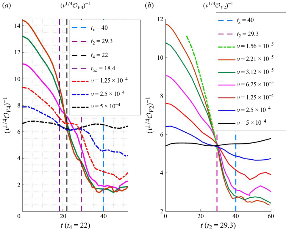
Figure 5. v^{1/4}O_{V_m} for m=2, 4 . Right legend shows the colours for all the \nu plotted in both frames. Both frames show t_1 = t_x = 40 , the end of the reconnection phase, and t_2 = 29.3 . (a) v^{1/4}O_{V4} for t \leq 50 . Also marked are t_4 \sim 22 and t_\infty \sim 18.4 with t_x > t_2 > t_4 > t_\infty . For \nu \leq 6.25 \times 10^{-5} , the v^{1/4}O_{V4}(t) converge at t_4 and for \nu \geq 1.25 \times 10^{-4} in -\infty , the convergence is around t_2 (b) All v^{1/4}O_{V2} for t \leq 60 , including \nu = 1.56 \times 10^{-5} , converge at t_2 = 29.3 .
