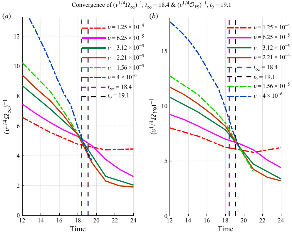
Figure 4. (a) (\nu^{1/4}\Omega_\infty)^{-1} and (b) (\nu^{1/4}\mathcal{O}_{V9})^{-1} with (1.9) showing how each \mathcal{O}_{V9} is bounded by V_\ell^{1/2m}\Omega_\infty (1.9). Outliers, indicated by dash-dotted lines, are under-resolved \nu < 2.21 \times 10^{-5} and a delayed crossing for \nu = 1.25 \times 10^{-4} . Recall that the end of the reconnection phase is indicated by when the \sqrt{\nu}Z(t) converge at t_x = 40 in figure 3. For \nu = 6.25 \times 10^{-5} to \nu = 4 \times 10^{-6} , in panel (a), the (\nu^{1/4}\Omega_\infty(t))^{-1} converge at t_\infty \sim 18.4 and in panel (b), the (\nu^{1/4}\mathcal{O}_{V9})^{-1} converge at t_9 \sim 19.1 .
