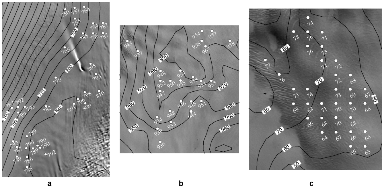
Fig. 4. Three regions of the ice stream (a–c; see Fig. 2 for locations) where enough matches for the old pair of images (1989–2000, white circles) allow a significant comparison with the velocity contours from the recent pair (2000–2001). The two first subscenes (a, b), along the main tributary, show an increase in velocity of around 30 \text{ m a}^{-1} ; the third (c), in a slow-moving part of the glacier, shows no change in velocity.
