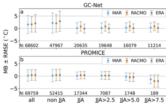
Figure 8. Mean bias (MB) and root-mean-square error (RMSE) in 2 m air temperature between models (MAR, RACMO and ERA5) and the (a) GC-Net and (b) PROMICE climate networks computed over the whole study period (all), over the period between September and May (non JJA), over the summer (JJA) and over the summer but using only days with average wind speed greater than 2.5, 5.0 or 7.5 m s -1 (e.g. JJA > 2.5 m s -1 , etc.). Sample number ( N ) is shown at the bottom of each plot.
