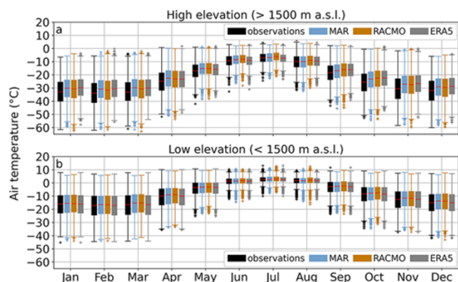
Figure 7. Boxplot of monthly 2m air temperature from observations and models (MAR, RACMO and ERA5) at (a) high elevation sites and (b) low elevation sites. Median is shown with a red line, 1st and 3rd quartiles with a box, lower and upper whiskers with colored lines and outliers as a cross.
