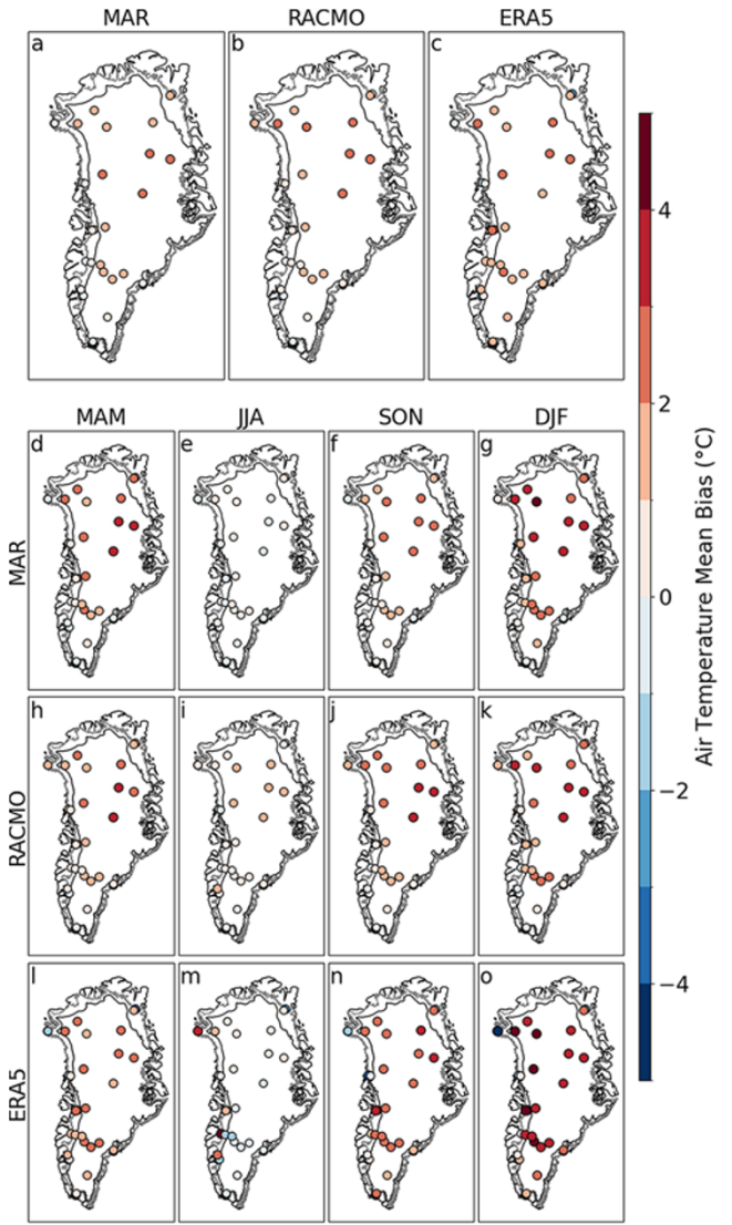
Figure 3. Maps of mean bias in 2 m air temperature in (a, d–g) MAR, (b, h–k) RACMO and (c, l–o) ERA5 compared to daily observations at 35 sites (a–c) over the entire study period and (d–o) for four seasons. The 1500 m contour (black line) is from the ArcticDEM (Porter and others, 2018) and the ice sheet extent (gray line) is based on Howat and others (2014).
