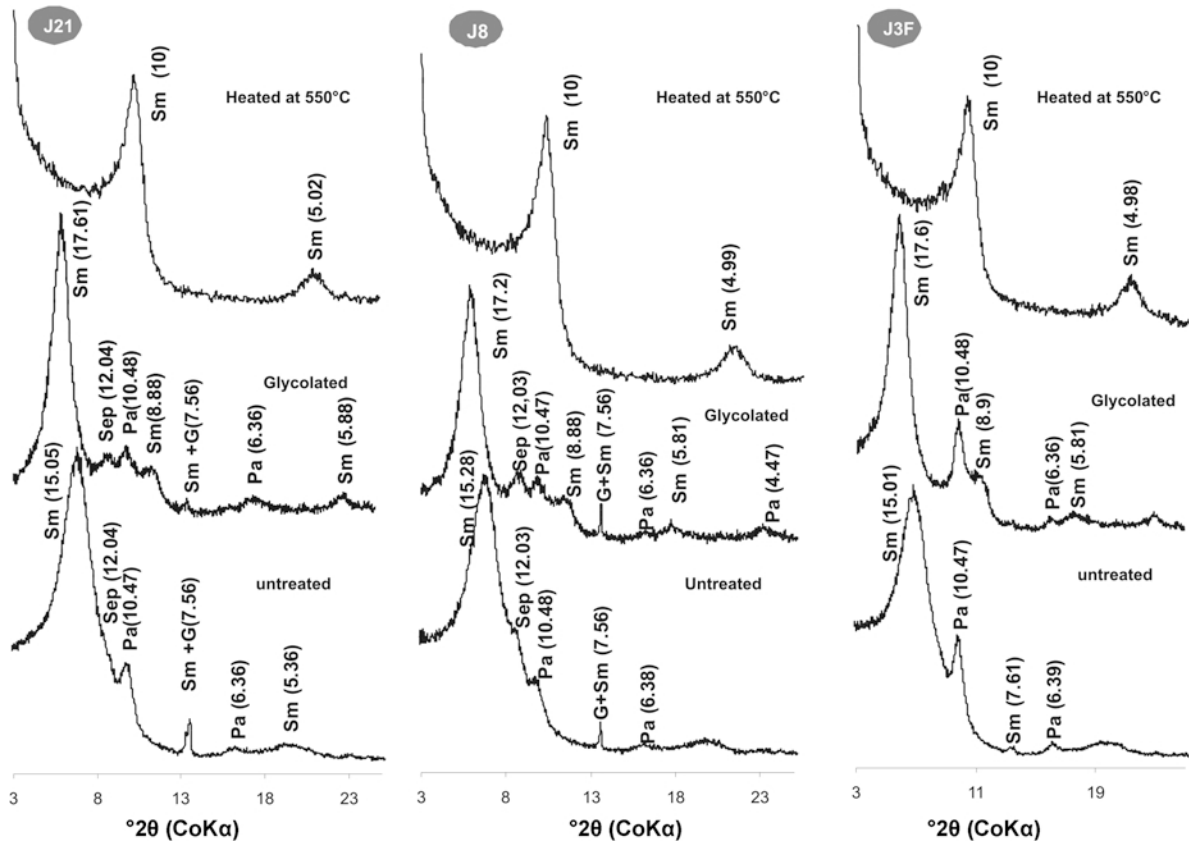
Figure 5. XRD patterns (CoKα radiation) of three oriented clay fractions of the samples J21, J8, and J3F (Sm: smectite; Sep: sepiolite; Pa: palygorskite, G: gypsum).
