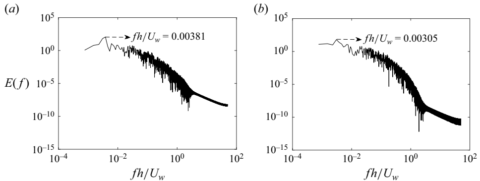
Figure 12. Frequency-based representation of streamwise velocity u for (a) d-type roughness ( Re = 350 ) and (b) k-type roughness ( Re = 300 ).
