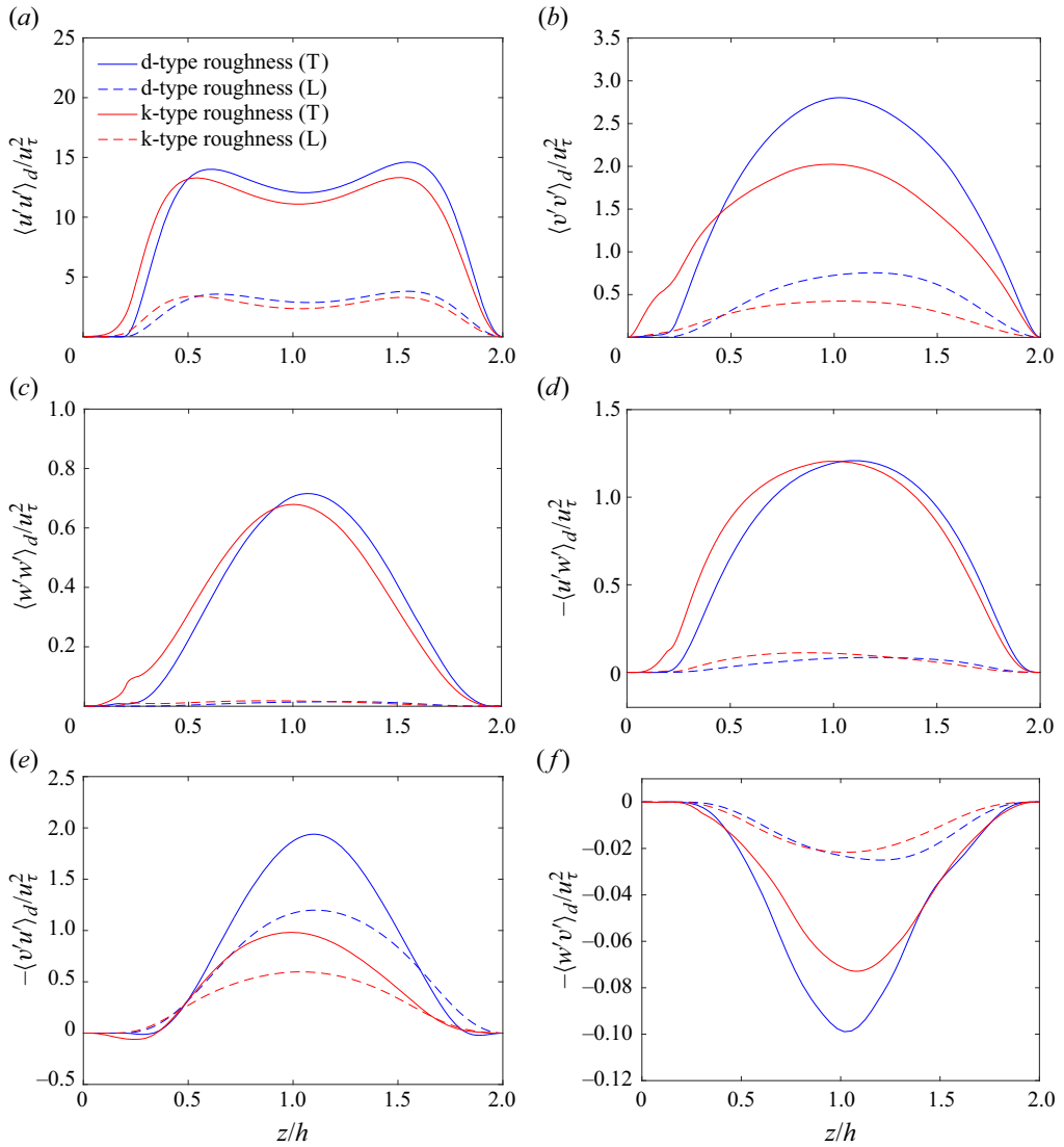
Figure 26. Wall-normal variation of \langle u'_i u'_j \rangle_d for the rough pCf cases at a Reynolds number close to their Re_g . The values are normalised using u_\tau^2 of each case. The legend labels (T) and (L) indicate the turbulent and quasi-laminar regions, respectively.
