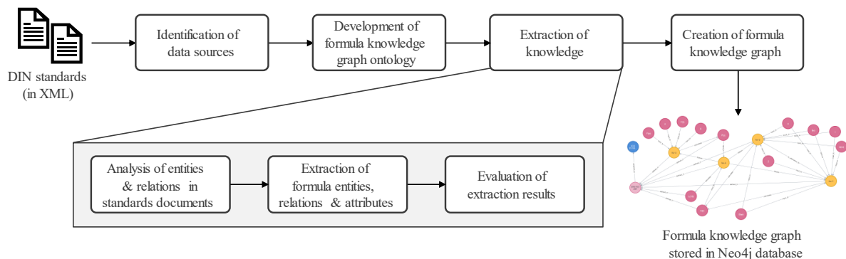
Figure 1. Process for automatic formula KG creation
