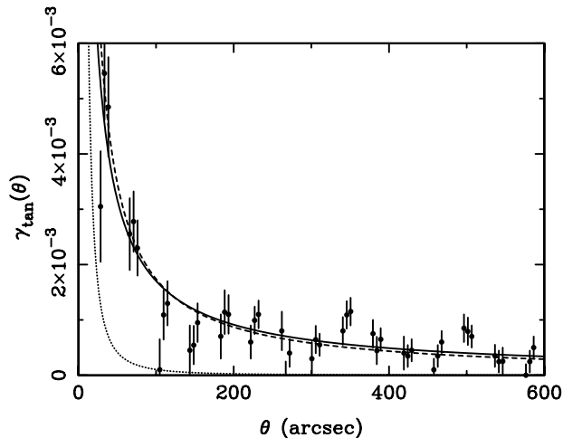
Figure 1 The mean shear, \gamma_{\text{tan}}(\theta) , around foreground galaxies in the g' , r' and i' bands, as measured by Fischer et al. (2000), is compared to various theoretical predictions. In each bin the data in the three bands (which are offset for clarity) are strongly correlated as the errors are dominated by the sample noise in the orientations of the background galaxies. The three models shown are: the best-fit power law (solid line); the MONDian prediction (dashed line); and the Newtonian result if there is no dark matter (dotted line).
