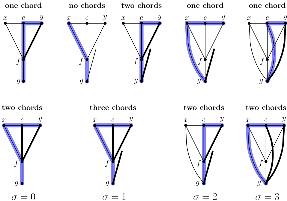
Figure 4. Proof of Claim 4.10.
