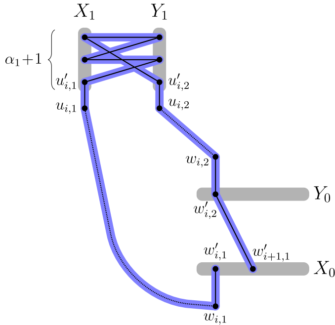
Figure 11. The path Q_i in Case (1).
