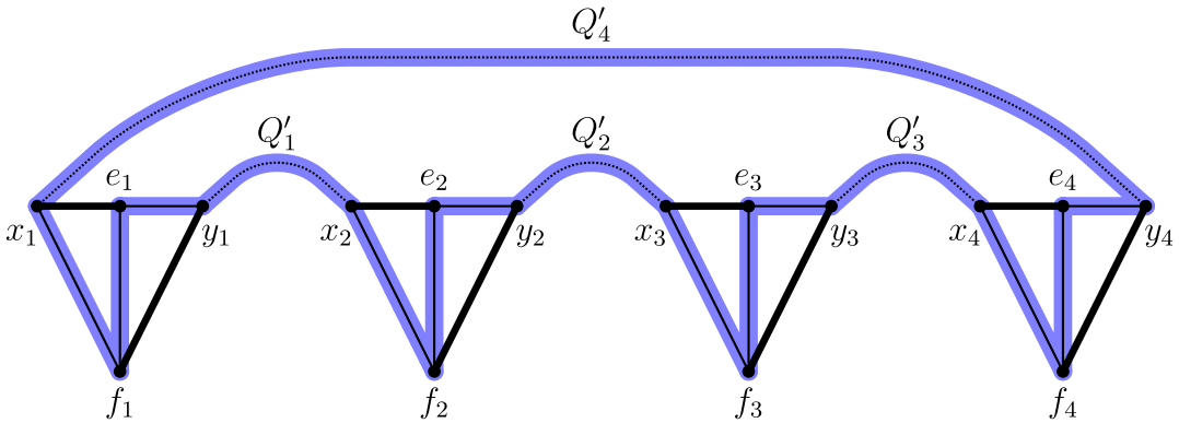
Figure 3. Case 2: k even f_i adjacent to x_i and y_i .
