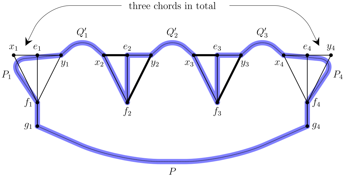
Figure 5. Case 3: odd k and f_i adjacent to x_i and y_i .
