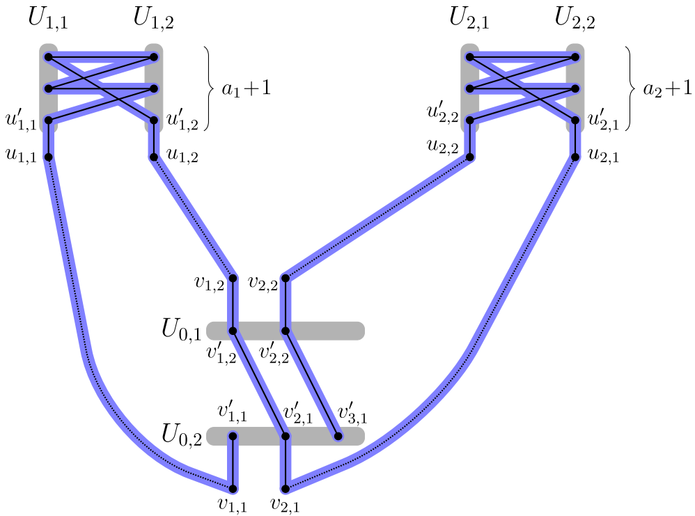
Figure 8. Part of the cycle \mathcal{C}(a_1, \dots, a_{100}) .
