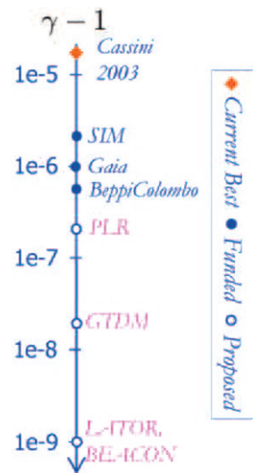
Figure 2. Anticipated progress in the tests of the PPN parameter \gamma (Turyshev 2009a).
