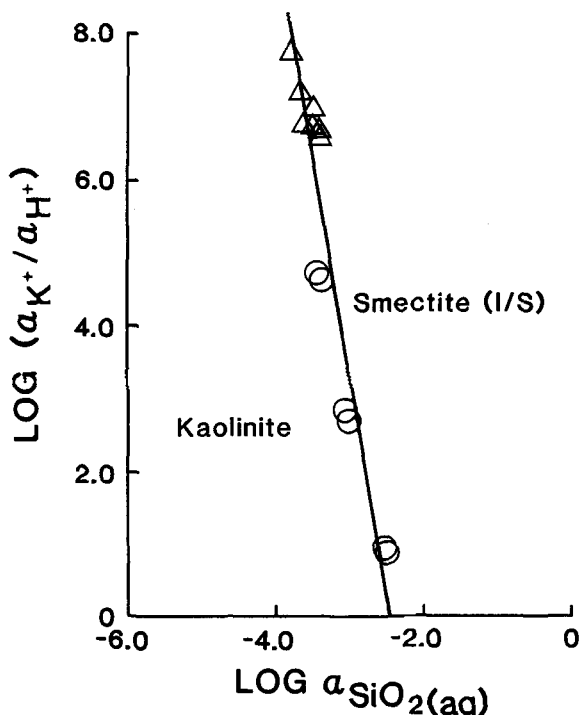
Figure 1. Compositions of solutions equilibrated with Goose Lake illite + kaolinite; triangles, Sass (1984); circles, Kittrick (1984). Smectite (I/S), smectite component of I/S.
