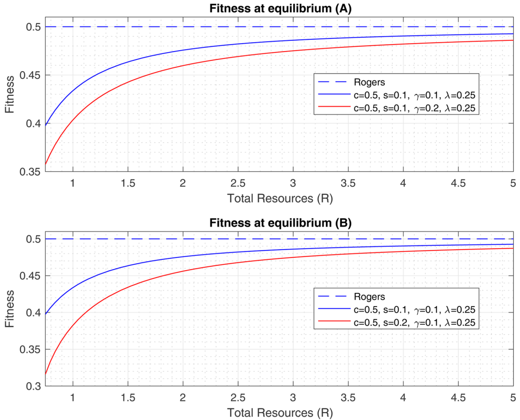
Figure 2. Fitness at equilibrium as a function of the expected population level resources, R . The dashed blue line shows Rogers' equilibrium fitness (invariant to all parameters but c ), the solid blue lines represent the baseline of c=0.5 , \lambda=0.25 , \gamma=0.1 , and s=0.1 and the red line depicts (A) a 0.1 increase in \gamma and (B) a 0.1 increase in s .
