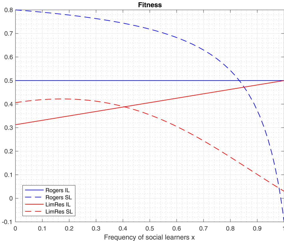
Figure 3. Fitness of individual and social learners as a function of social learners' frequency. In this example \gamma=0.10 , c=0.50 , s=0.10 , R=0.60 , \lambda=0.17 , z=0.50 and \omega=0.25 . Blue lines are the guaranteed resources model (Rogers) and red lines are the uncertain resources model with semi-tuned agents. The ESS frequency is at the intersection of individual learning and social learning curves.
