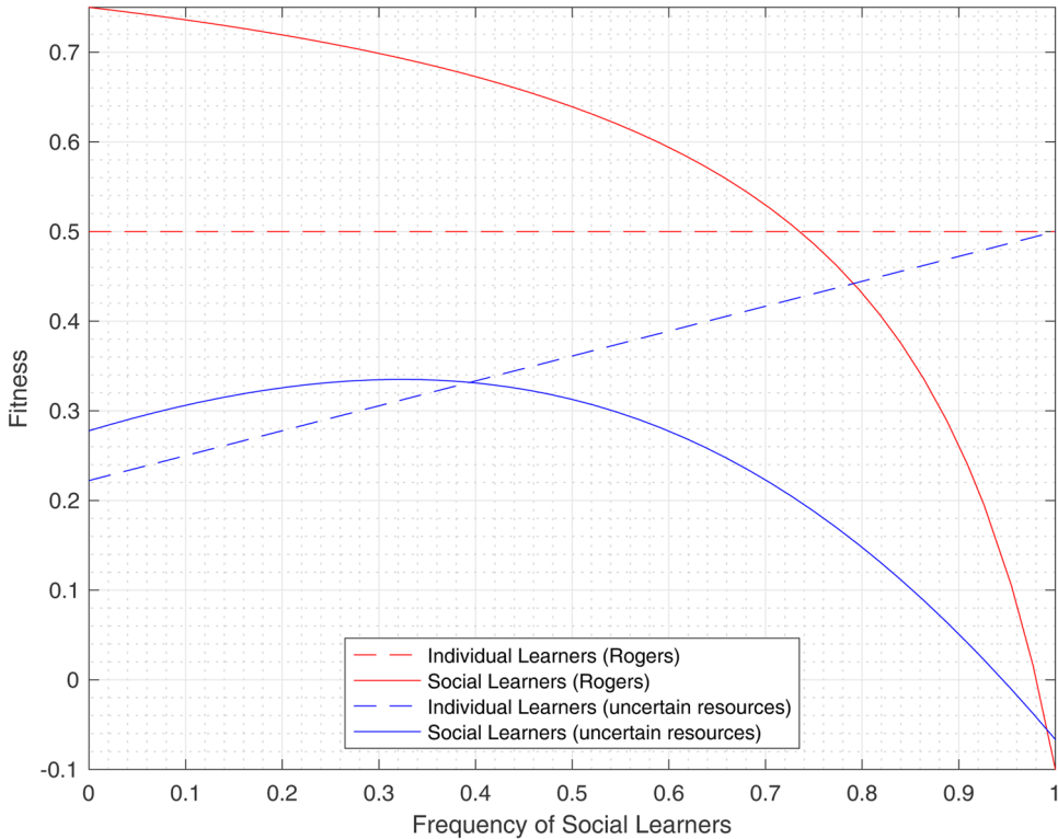
Figure 1. Fitness of individual and social learners as a function of social learners’ frequency. In this example \gamma=0.10 , c=0.50 , s=0.20 , R=0.60 and \lambda=0.25 . Red lines are the guaranteed resources model (Rogers) and blue lines are the uncertain resources model. The ESS frequency is at the intersection of individual learning and social learning curves.
