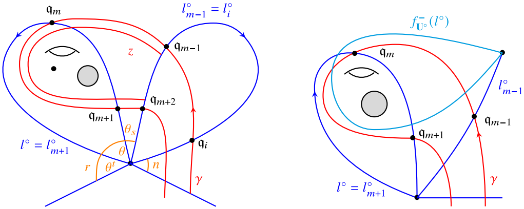
Figure 20. The case l^\circ = l_{m+1}^\circ .
