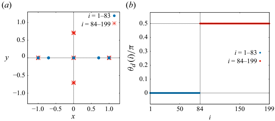
Figure 11. (a) Rescaled configurations of the five \alpha -point vortices at t_c^\varepsilon(\theta_i) . (b) Angle between the diagonals l_{12}^{\varepsilon_3}(t_c^\varepsilon; \theta_i) and l_{34}^{\varepsilon_3}(t_c^\varepsilon; \theta_i) divided by \pi .
