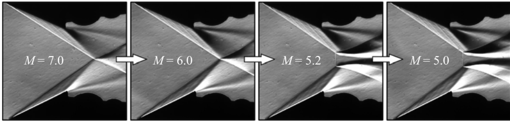
Figure 8. The RR \rightarrow MR hysteresis cycle induced by free-stream disturbances during Mach-number variation for \theta = 25^\circ , 2g = 40 mm and Re' = 4.5 \times 10^6 \text{ m}^{-1} (also see Supplementary Movie 3).
