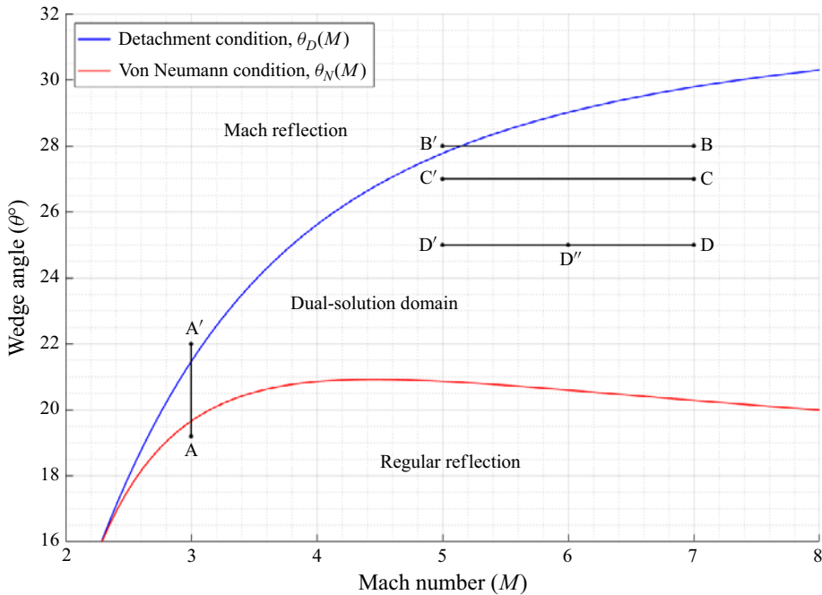
Figure 2. Dual-solution domain with hysteresis paths shown: AA'A, BB'B, CC'C, DD'D.
