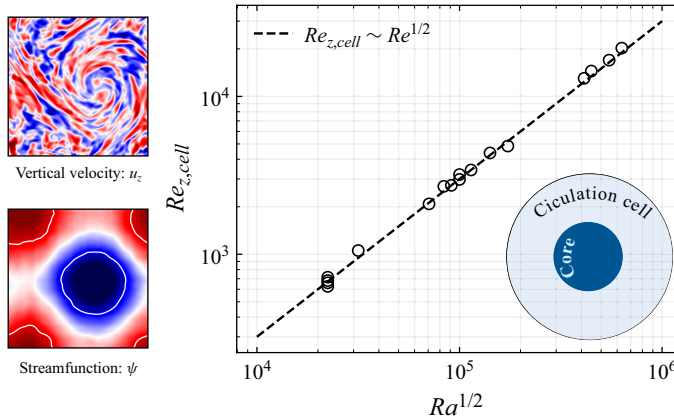
Figure 6. Left-hand column: instantaneous u_z and \psi contours at mid-plane for a large-scale vortex at Ra = 2 \times 10^{11} , Pr = 1 , Ek = 5 \times 10^{-8} (red/blue for positive/negative values; white line at \psi = 0.8\psi_{max} marks vortex core). Right-hand column: Re_{z,cell} in the circulation cell ( |\psi| \leq 0.8\psi_{max} ) versus Ra^{1/2} . Inset: schematic of vortex core and circulation cell.
