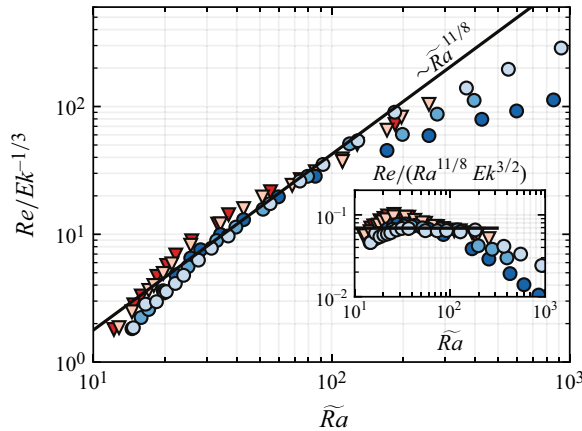
Figure 5. Dimensionless momentum transport Re , normalised by Ek^{-1/3} , versus supercriticality \tilde{Ra} = Ra Ek^{4/3} for stress-free (circles) and no-slip (triangles) RRBC. Inset: Re , normalised by (3.7), in the diffusion-free heat transfer regime, versus \tilde{Ra} . A power-law fit to stress-free DNS data for 40 \leq \tilde{Ra} \leq 200 gives Re \sim \tilde{Ra}^\alpha at fixed Ek , with \alpha = 1.26 \pm 0.14 (95 % confidence interval), which supports (3.7) and which is clearly different from the diffusion-free scaling for no-slip boundary condition as shown in figure 2(b).
