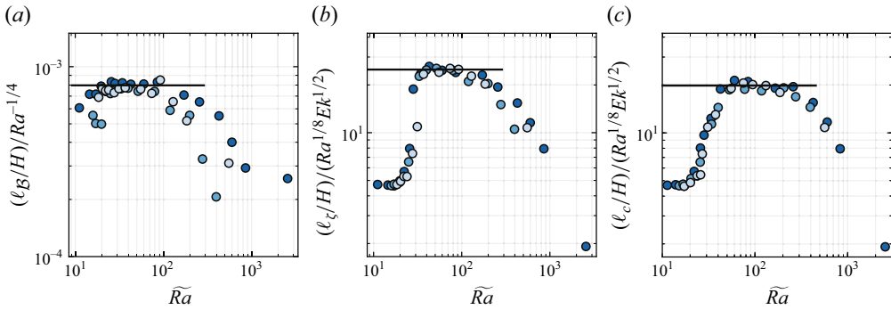
Figure 4. The background convective length scale \ell_B , representing the spatial extent of the circulation region. (b) The characteristic convective length scale \ell_z , derived from vertical vorticity \omega_z . (c) The convective length scale \ell_c , based on vertical velocity. All are normalised by the new scaling laws proposed in (3.2) and (3.5), within the diffusion-free heat transfer regime. These are plotted as functions of \tilde{Ra} = Ra Ek^{4/3} . A power-law fit to the DNS data in the moderate range 40 \leq \tilde{Ra} \leq 200 yields the scaling relation Re \sim \tilde{Ra}^\alpha at fixed Ek , with fitted exponents \alpha for (a) \ell/H = 0.23 \pm 0.12 , (b) \ell_z/H = 0.11 \pm 0.09 and (c) \ell_c/H = 0.12 \pm 0.05 (95 % confidence interval), supporting the scaling relations presented in (3.2) and (3.5).
