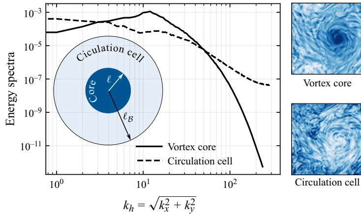
Figure 3. Okubo–Weiss decomposition of barotropic energy at Ra = 2 \times 10^{11} , Ek = 5 \times 10^{-8} , with spectra for vortex core (solid line) and background circulation cell (dashed line). Vortex core and circulation cell length scales, \ell and \ell_B , are shown in the inset schematic. Right-hand column: contour plots of horizontal vorticity (vortex core) and strain (circulation cell), with dark/light colours for high/low values.
