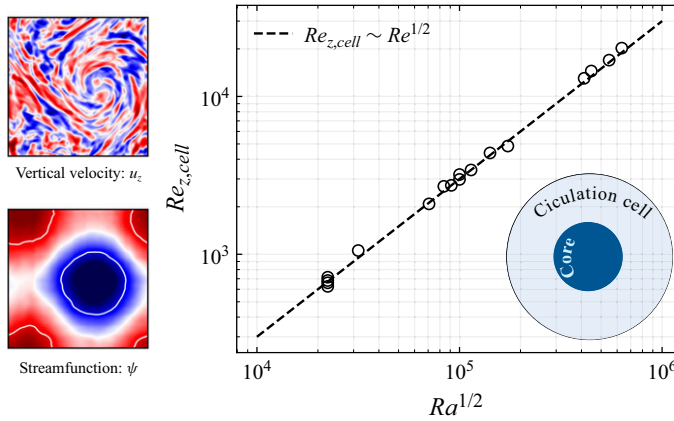
Figure 6. Left-hand column: instantaneous u_z and \psi contours at mid-plane for a large-scale vortex at Ra = 2 \times 10^{11} , Pr = 1 , Ek = 5 \times 10^{-8} (red/blue for positive/negative values; white line at \psi = 0.8\psi_{max} marks vortex core). Right-hand column: Re_{z,cell} in the circulation cell ( |\psi| \leq 0.8\psi_{max} ) versus Ra^{1/2} . Inset: schematic of vortex core and circulation cell.
