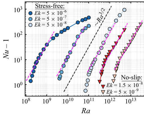
Figure 1. Dimensionless convective heat transport Nu - 1 as a function of the Rayleigh number Ra for various Ekman numbers Ek , obtained from DNS of RRBC with stress-free and no-slip boundary conditions at Pr = 1 . The dashed lines represent the heat transfer scaling for geostrophic turbulence, Nu - 1 \sim Ra^{3/2} .
