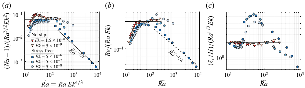
Figure 2. (a) Nusselt number Nu - 1 , normalised by the diffusion-free scaling Ra^{3/2} Ek^2 . (b) Dimensionless momentum transport Re , normalised by its geostrophic turbulence scaling Ra Ek . (c) Dimensionless convective length scale \ell_c/H , normalised by its geostrophic turbulence scaling Ra^{1/2} Ek , shown as a function of the supercriticality parameter \tilde{Ra} \equiv Ra Ek^{4/3} and increasing supercriticalities.
