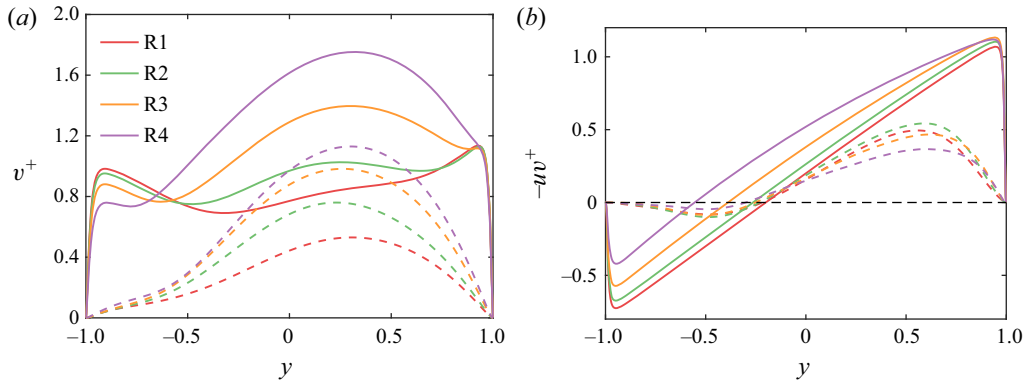
Figure 12. (a) Root-mean-square profiles of wall-normal velocity fluctuations and (b) profiles of the mean turbulent shear stress \overline{uv} in global scaling. The solid lines show the unfiltered results and the dashed lines the contribution of the large-scale motions.
