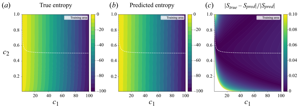
Figure 4. (a) True entropy. (b) Predicted entropy given by OB model in (3.1). (c) Relative error in the prediction of the entropy for the PINN-rheometric model.
