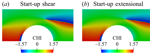
Figure 25. Orientation angle ( \chi ) for flow around a cylinder at Wi = 0.2 .
