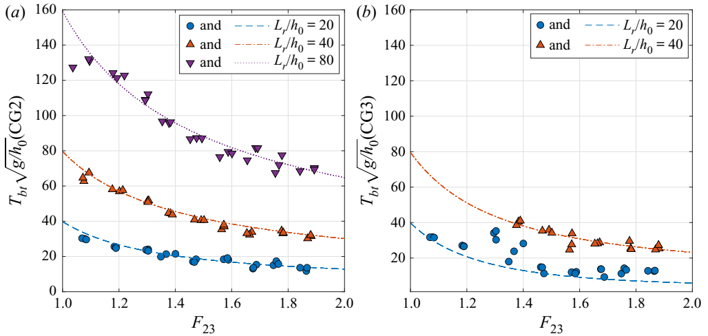
Figure 15. The bore periods measured at CG2 on panel (a), and CG3 on panel (b), for different reservoir lengths. Markers represent experimental data. Lines are calculated using (4.2) by substituting the input parameters ( F_{in} , L_r ) at CG2 and CG3, where x_t is the location of the respective CG (see table 1).
