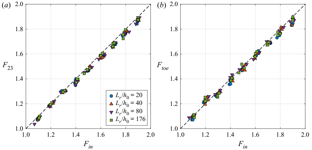
Figure 7. Measured bore strengths between CG2 and CG3 (a), and between CG3 and CG4 (b), for different reservoir length and bore strength. The dashed line represents the theoretical bore strength.
