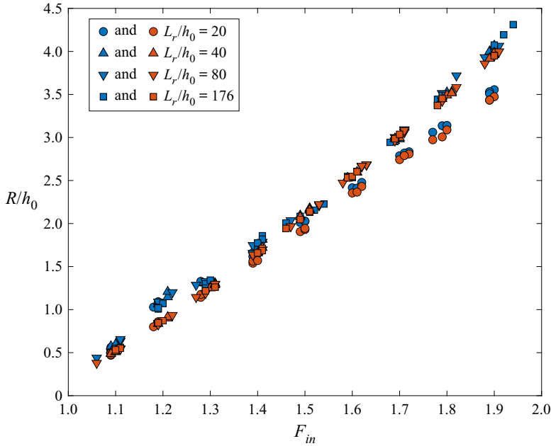
Figure 19. Dimensionless maximum run-up heights, R/h_0 , in terms of the input bore strength, F_{in} . Blue markers represent laboratory experiments and orange markers symbolize the numerical simulations for the same input parameters.
