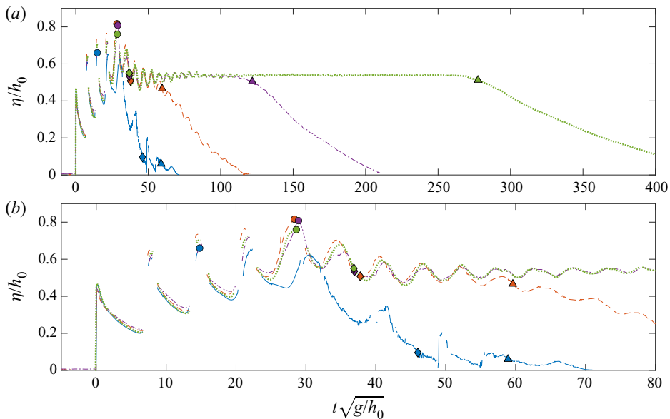
Figure 9. Time histories of dimensionless free surface elevations at the still-water shoreline are shown for undulating bore with strength of F_{in} = 1.2 . (a) The time histories for a longer period of times are shown, while the details of the bore front are shown in panel (b). Results: L_r/h_0 = 20 (blue line); L_r/h_0 = 40 (orange line); L_r/h_0 = 80 (purple line); L_r/h_0 = 176 (green line). Circles represent the maximum free surface height ( I/h_0 ); diamonds represent the beginning of the flooding plateau and triangles the end of the flooding plateau.
