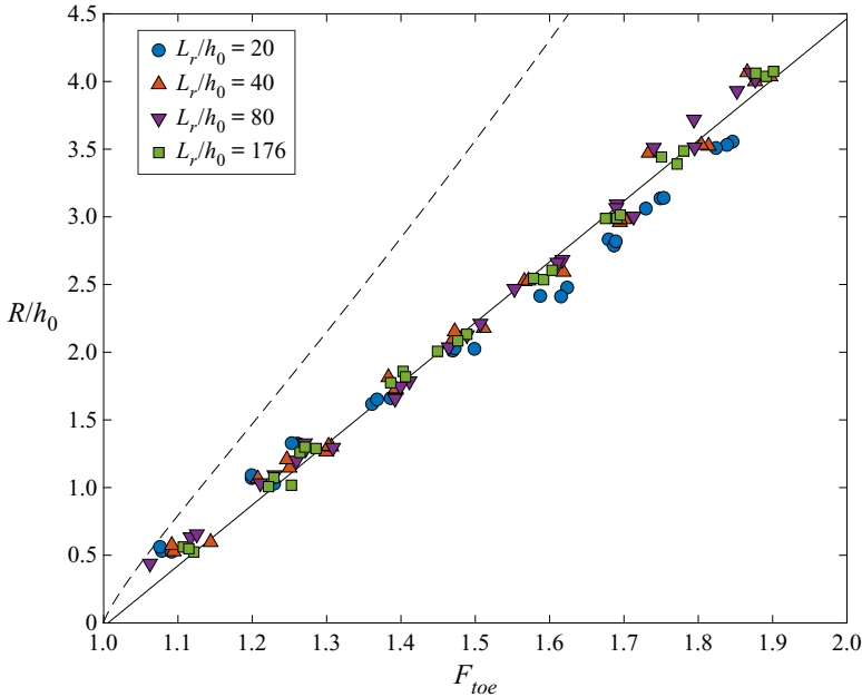
Figure 13. Dimensionless maximum run-up, R/h_0 , in terms of the bore strength at the beach toe, F_{toe} and the reservoir length, L_r/h_0 . The solid black line represents the predictive solution (5.4) and the dashed line represents Shen & Meyer (1963) run-up solution.
