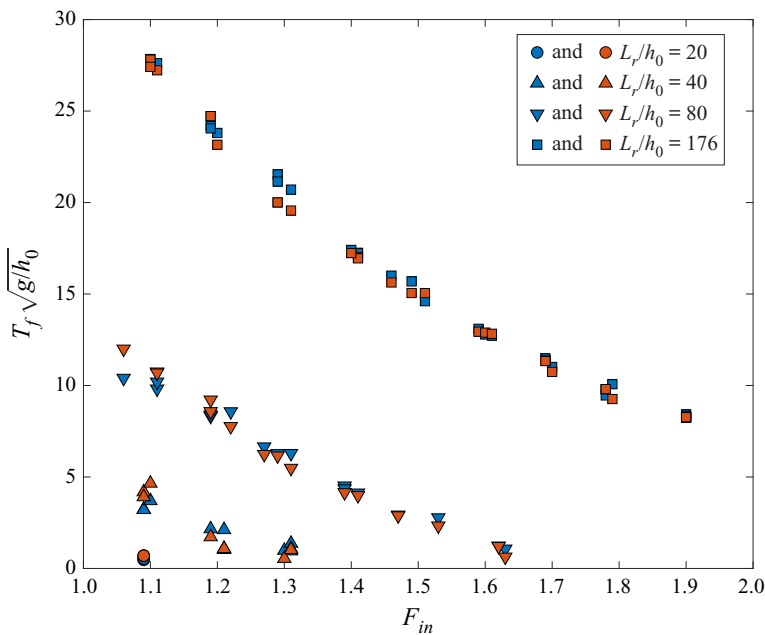
Figure 20. Dimensionless flooding duration at the still-water shoreline, T_f \sqrt{g/h_0} , in terms of the input bore strength, F_{in} . Blue markers represent laboratory experiments and orange markers symbolize the numerical simulations for the same input parameters.
