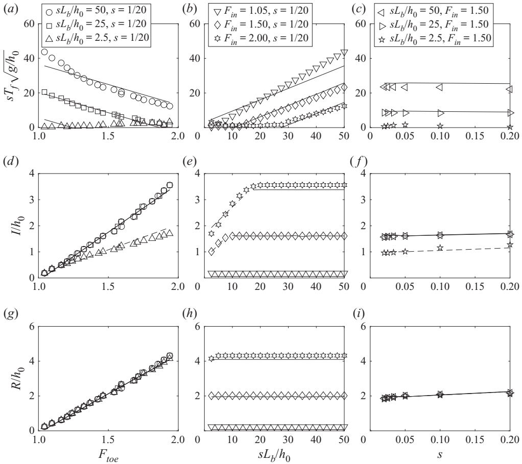
Figure 16. (a–c) Flooding duration ( sT_f/\sqrt{g/h_0} ); (d–f) maximum inundation at the still-water shoreline ( I/h_0 ); (g–i) maximum run-up height ( R/h_0 ). (a,d,g) Numerical results are plotted against the bore strength at the beach toe ( F_{toe} ); (b,e,h) the target bore length ( sL_b/h_0 ) at the beach toe; (c,f,i) the slope ( s ). Solid lines on panels (a–c) represent the predictive equation (5.5). Solid lines on panels (d–f) represent predictive equation (5.2) and dashed lines (5.1). Solid lines on panels (g–i) represent predictive equation (5.4).
