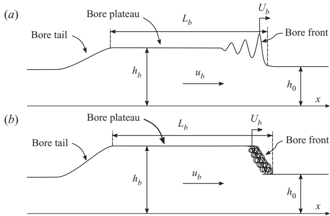
Figure 1. Definition sketch for a bore of limited length propagating on a horizontal bed. (a) Undulating bore and (b) breaking bore.
