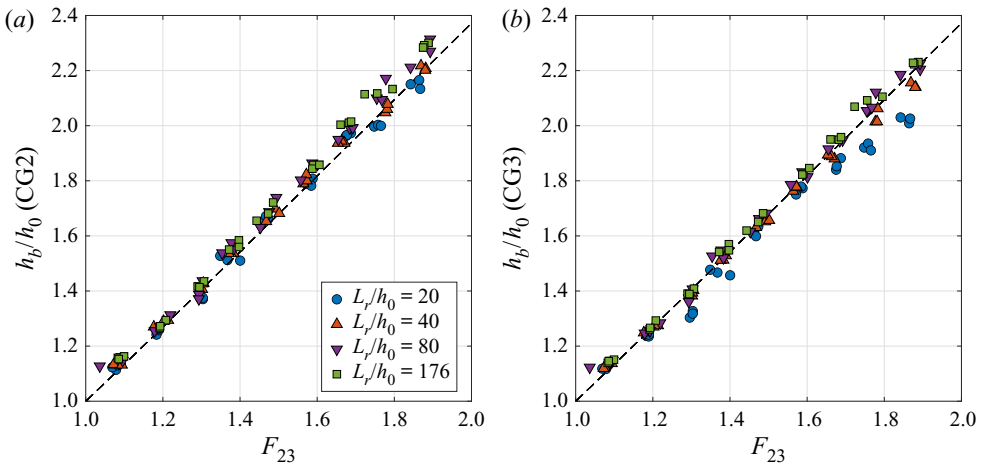
Figure 8. Measured bore heights at CG2 (a), and at CG3 (b) for different reservoir length and measured bore strengths. The dashed line represents the theoretical bore height correspondent to a given bore strength (2.3).
