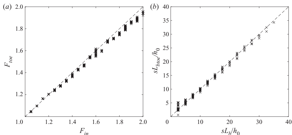
Figure 21. Numerical results for the parametric analysis simulations: (a) bore strength at the beach toe versus the input target bore strength; (b) the bore lengths at the time when the bore reaches the beach toe versus the input target bore lengths at the beach toe. The coefficient of determination is R^2 = 0.984 for panel (a) and R^2 = 0.987 for the panel (b).
