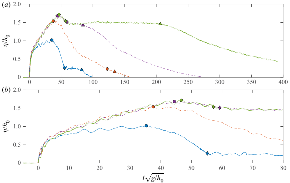
Figure 10. Time histories of dimensionless free surface elevations at the still-water shoreline are shown for undulating bore with strength of F_{in} = 1.5 . (a) The time histories for a longer period of times are shown, while the details of the bore front are shown in panel (b). Results: L_r/h_0 = 20 (blue line); L_r/h_0 = 40 (orange line); L_r/h_0 = 80 (purple line); L_r/h_0 = 176 (green line). Circles represent the maximum free surface height ( I/h_0 ); diamonds represent the beginning of the flooding plateau and triangles the end of the flooding plateau.
