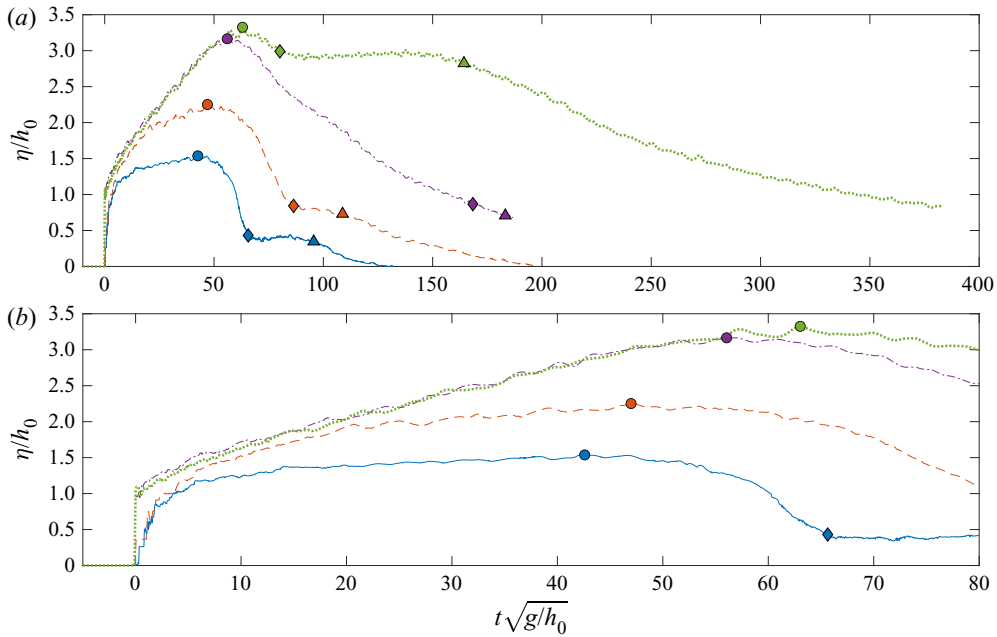
Figure 11. Time histories of dimensionless free surface elevations at the still-water shoreline are shown for undulating bore with strength of F_{in} = 1.9 . (a) The time histories for a longer period of times are shown, while the details of the bore front are shown in panel (b). Results: L_r/h_0 = 20 (blue line); L_r/h_0 = 40 (orange line); L_r/h_0 = 80 (purple line); L_r/h_0 = 176 (green line). Circles represent the maximum free surface height ( I/h_0 ); diamonds represent the beginning of the flooding plateau and triangles the end of the flooding plateau.
