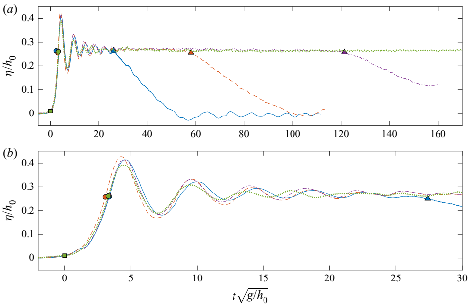
Figure 4. Time histories of dimensionless free surface elevations at CG2 for undulating bore with strength of F_{in} = 1.2 . Two views are presented: while the zoomed-out view is shown in panel (a), the details of the bore front are shown in panel (b). Results: L_r/h_0 = 20 (blue line); L_r/h_0 = 40 (orange line); L_r/h_0 = 80 (purple line); L_r/h_0 = 176 (green line). Squares represent the arrival of bore front, triangles the beginning of tail and circles the first measurement with bore height equal to or larger than the bore height at the beginning of the bore tail.
