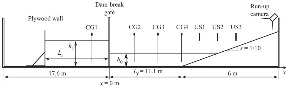
Figure 3. Dam-break experimental set-up in the NUS hydraulic laboratory (not to scale).
