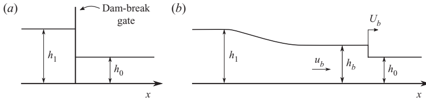
Figure 2. (a) Initial conditions of a dam-break system. (b) Representation of the generated bore.
