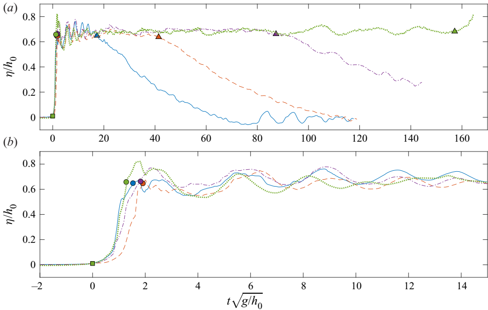
Figure 5. Time histories of dimensionless free surface elevations at CG2 for undulating bore with strength of F_{in} = 1.5 . Two views are presented: while the zoomed out view is shown in panel (a), the details of the bore front are shown in panel (b). Results: L_r/h_0 = 20 (blue line); L_r/h_0 = 40 (orange line); L_r/h_0 = 80 (purple line); L_r/h_0 = 176 (green line). Squares represent the arrival of bore front, triangles the beginning of tail and circles the first measurement with bore height equal to or larger than the bore height at the beginning of the bore tail.
