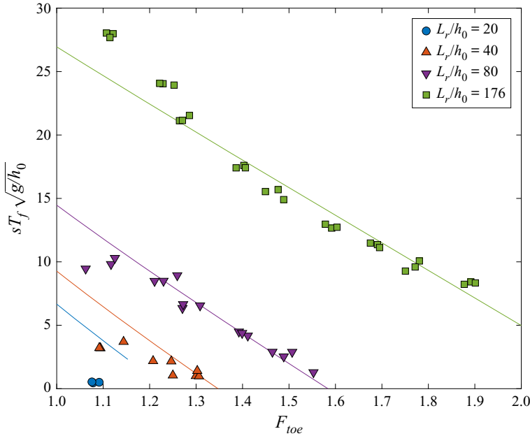
Figure 14. Dimensionless flooding duration at the still-water shoreline, sT_f\sqrt{g/h_0} , in terms of the bore strength at the beach toe, F_{toe} , and the reservoir length, L_r/h_0 . The solid coloured lines represent the predictive solution (5.5), in which L_b is calculated using (4.5).
