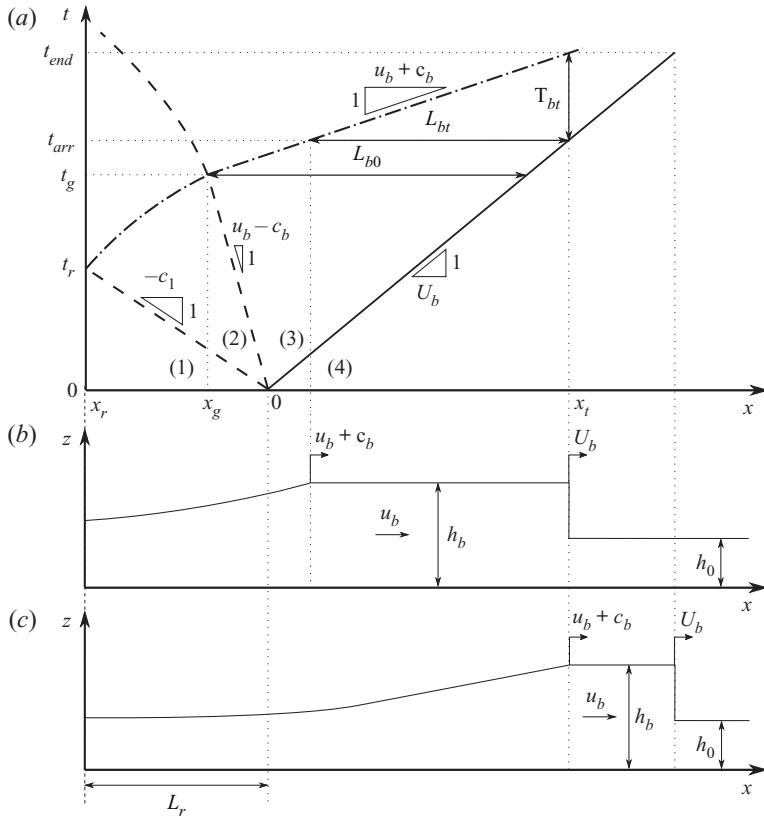
Figure 17. (a) Sketch of the characteristics plane of a bore generated by a dam-break system with a reservoir length L_r , whose gate opens at (0, 0) . The continuous line represents the bore front propagation, dashed lines represent two negative characteristics departing from the gate (a trough propagating upstream with velocity c_1 and the end of the bore plateau propagating with velocity u_b - c_b ) and dashed-dotted lines denote the positive characteristics reflected from the back wall of the reservoir at time t_r . The initial bore length ( L_{b0} ) is defined at the time at which the reflected positive characteristic meets the end of the bore plateau at (x_g, t_g) . (b,c) Two-dimensional vertical representation of the generated bore at time t_{arr} and t_{end} , respectively.
