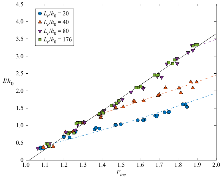
Figure 12. Dimensionless inundation depths at the still-water shoreline, I/h_0 , in terms of the bore strength measured at the beach toe, F_{toe} , and the reservoir length, L_r/h_0 . The black solid line represents the predictive equation (5.2) and the dashed coloured lines equation (5.1), in which L_b is calculated using (4.5).
