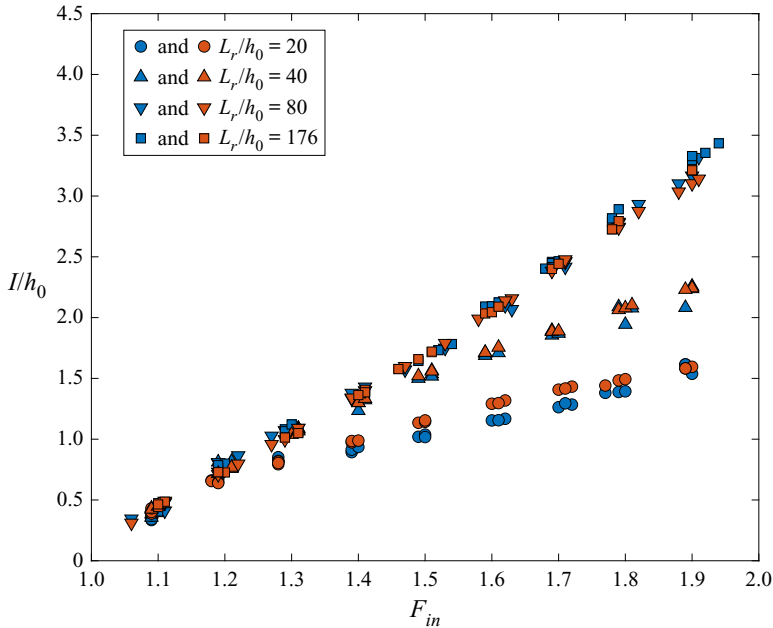
Figure 18. Dimensionless inundation depths at the still-water shoreline, I/h_0 , in terms of the input bore strength, F_{in} . Blue markers represent laboratory experiments and orange markers symbolize the numerical simulations for the same input parameters.
