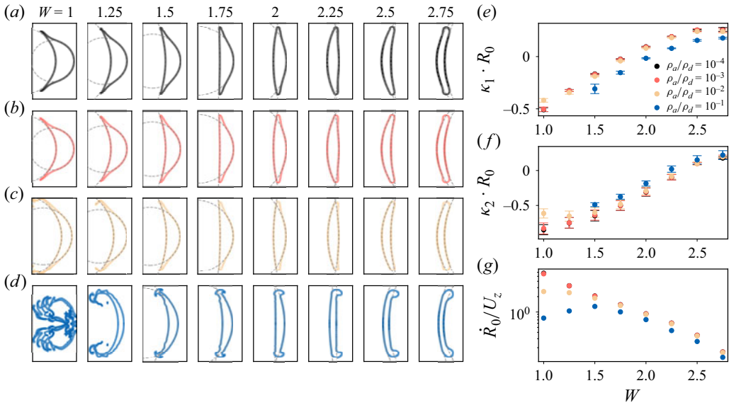
Figure 12. Effect of the density ratio in the sheet curvature at time t = R_0 / \dot{R}_0 . The values Re = 1000 , We = 1000 , \mu_a/\mu_d = 10^{-4} are kept fixed, and a sweep is performed in the density ratio and pressure profile parameter W . Almost no effects are observed for the two smaller values of density ratio. For the higher values, significant drag is present, particularly for the cases with small W , resulting in changes in the measured curvature and reducing expansion velocity.
