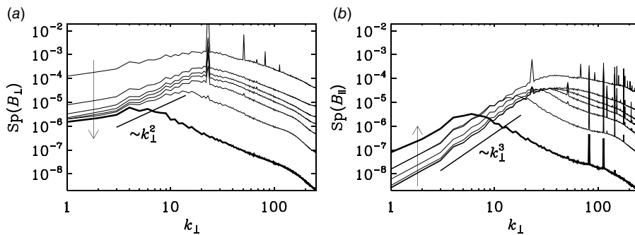
FIGURE 13. Spectra of (a) B_{\perp} and (b) B_{\parallel} as a function of k_{\perp} in both panels. The last time is shown as a thick line. The sense of time is also shown by the arrows in both panels.
