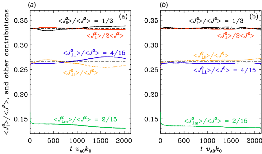
FIGURE 10. Evolution of \langle J_{\perp}^2 \rangle / \langle J^2 \rangle (green), \langle J_{\perp\perp}^2 \rangle / \langle J^2 \rangle (blue), \langle J_{\parallel}^2 \rangle / \langle J^2 \rangle (orange), \langle J_{\perp}^2 \rangle / 2 \langle J^2 \rangle (red), and \langle J_{\parallel}^2 \rangle / \langle J^2 \rangle (black) for decaying isotropic turbulence with an initial peak wavenumber k_0/k_1 = 8 using 1024^3 meshpoints (a) with helicity and (b) without helicity.
