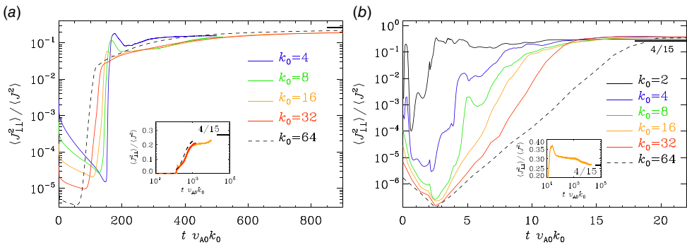
FIGURE 1. Evolution of \langle J^2_{\perp\perp} \rangle / \langle J^2 \rangle for (a) Roberts field I with k_0 = 4 (blue), 8 (green), 16 (orange), 32 (red) and 64 (black dashed), and for (b) Roberts field II with k_0 = 2 (black), 4 (blue), 8 (green), 16 (orange), 32 (red) and 64 (black dashed). The short thick line on the upper right indicates the value of 4/15 , which is reached only at much later times outside this plot. The insets demonstrate that \langle J^2_{\perp\perp} \rangle / \langle J^2 \rangle \rightarrow 4/15 much later.
