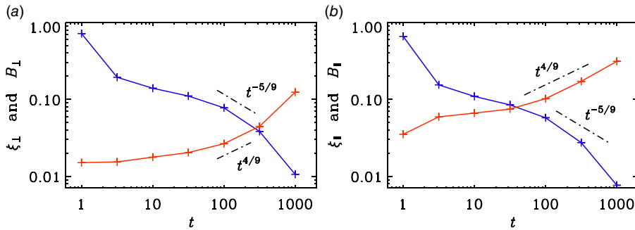
FIGURE 12. Scalings of (a) \xi_{\perp}(t) and B_{\perp}(t) , and (b) \xi_{\parallel}(t) and B_{\parallel}(t) in red and blue, respectively, both for the non-helical case. The expected slopes \propto t^{4/9} and \propto t^{-5/9} are indicated for reference.
