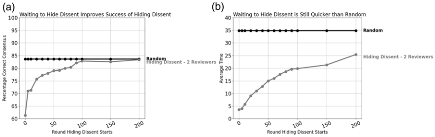
Figure 5. As the round where the scientists begin hiding dissent increases: (a) the percentage of times correct consensus is reached; (b) the average time until correct consensus. k = 4, r = 2, T = 100 .
