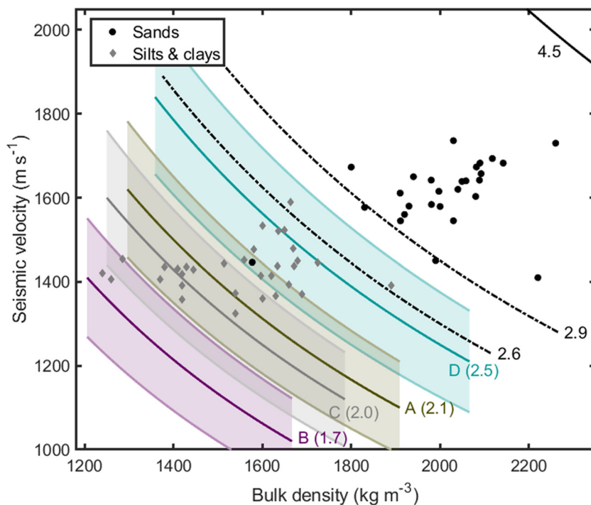
Figure 4. Seismic velocity and density for soft, wet subaqueous sediments for which the sediment composition is known (see Smith and others, 2018). Black circles are sands and sandy sediments, grey diamonds are silts and clays. Solid curves are the mean acoustic impedance values ( \times 10^6 \text{ kg m}^{-2} \text{ s}^{-1} ) for the different sections at the bed of SLC determined from the seismic data. Uncertainties in these measurements are presented by the respectively coloured patch. C covers the central part of the lake only; A, B and D also include the lake sides except for the strong dipping reflector which is represented by curve 4.5. As described in the text, in general, values below 2.6 \times 10^6 \text{ kg m}^{-2} \text{ s}^{-1} indicate silt- and clay-dominated sediments and above 2.9 \times 10^6 \text{ kg m}^{-2} \text{ s}^{-1} coarse, medium and fine sands and silty-sands.
