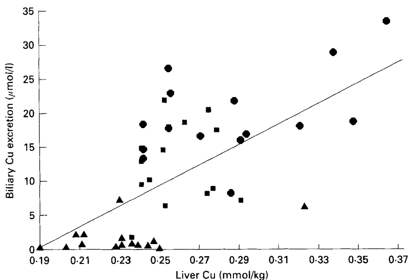
Fig. 4. Relationship between biliary Cu excretion and hepatic Cu concentration in individual rats fed on a low- (▲), normal- (■) or high- (●) Fe diet. The regression equation is y = 150x - 28 ( r 0.63, n 45, P < 0.05 ).
