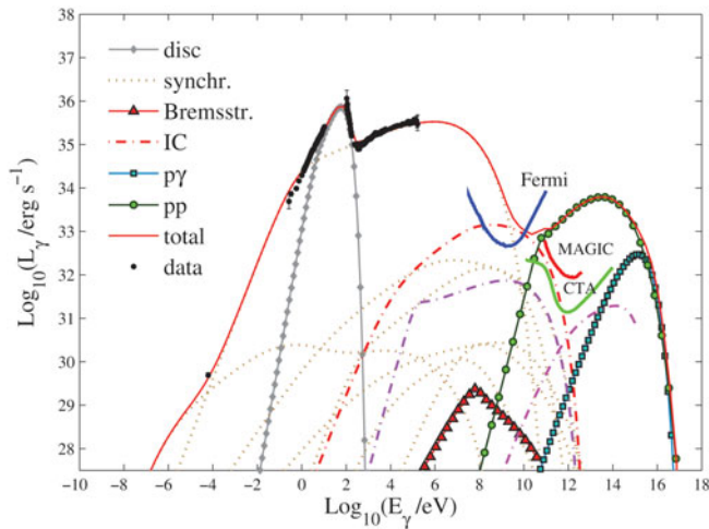
Figure 1. Spectral energy distribution of a flare that occurred in 2000 in the low mass microquasar XTE J1118+480. The data have been fitted with an inhomogeneous lepto-hadronic jet model. For details see Vila et al. (2012).
