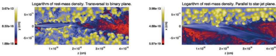
Figure 2. Axial cuts of rest-mass density of a simulated 3D jet propagating through a clumpy wind in a high-mass microquasar. A clear bend is seen in the jet direction. From Perucho & Bosch-Ramon (2012).
