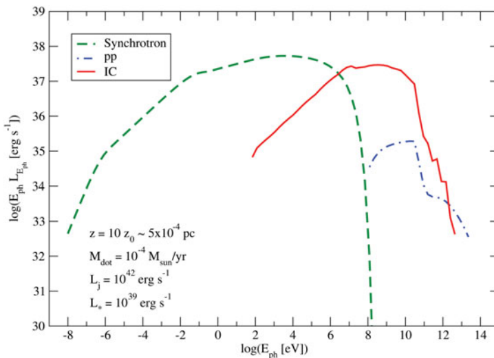
Figure 5. Spectral energy distribution of the radiation produced by a Wolf-Rayet star interacting with a relativistic jet of a Fanaroff-Riley I radio galaxy (Araudo et al. 2013).
