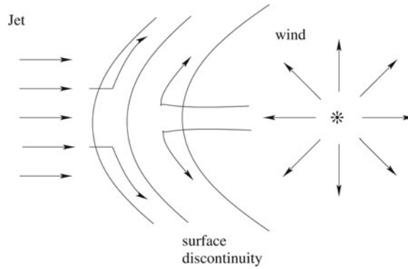
Figure 4. Schematic of a massive star interacting with a relativistic jet in an AGN. See Araudo et al. (2013) for details.
