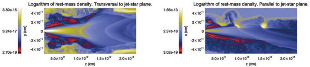
Figure 3. Axial cuts of rest-mass density of a simulated 3D jet interacting with massive clumps in a high-mass microquasar. From Perucho & Bosch-Ramon (2012).
