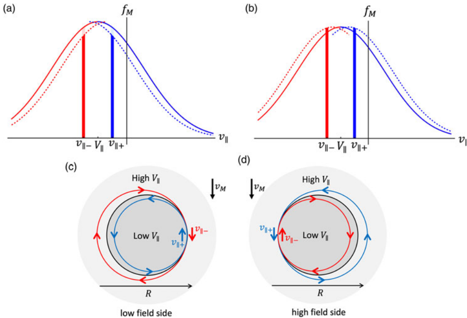
FIGURE 2. In this figure, we assume \partial V_{||}/\partial \psi > 0 . A blue (red) passing particle with parallel velocity v_{||+} > V_{||} = -u ( v_{||-} < V_{||} = -u ) on the low field side (a,c) or the high field side (b,d) is circulating in the positive (negative) sense in the poloidal direction. The solid lines represent the Maxwellian on the flux surface of interest. The dashed lines indicate the shifted Maxwellians radially inwards or outwards from the flux surface of interest. On the low field side, blue (red) particles complete their orbits through a region with smaller (larger) mean parallel flow (c), so their average radial position locates them in a region with fewer particles that have a parallel velocity close to v_{||+} ( v_{||-} ) (a). A point of slightly lower density develops on the outboard side. On the high field side, blue (red) particles complete their orbits through a region with larger (smaller) mean parallel flow (d), so their average radial position locates them in a region with more particles that have a parallel velocity close to v_{||+} ( v_{||-} ) (b). A point of slightly higher density develops on the high field side.
