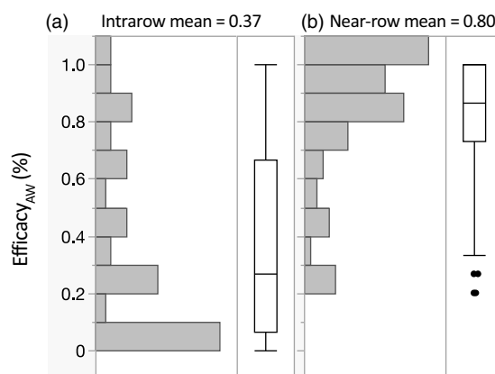
Figure 5. Efficacy based on scoring of artificial weeds measured in the 5-cm intrarow (A) and 5-cm near-row (B) zones in two soil bin experiments. Box plots show median center lines, upper and lower quartiles, with whiskers at 1.5× the interquartile; outliers are also shown.
