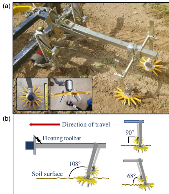
Figure 1. Finger weeder used in field and soil bin studies showing the spring-tensioned floating toolbar and angle adjustment mechanism (A) that allowed testing three different angles (B): 108° relative to the soil surface, angled toward the direction of travel; 90°, which is typical for most finger weeders; and 68°, angled away from the direction of travel.
