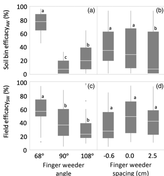
Figure 3. Finger weeder angle and spacing effects on intrarow efficacy measured with artificial weeds (Efficacy AW ) in the soil bin (A, B), and measured in the field using a surrogate weed (Efficacy SW ; Brassica juncea ). Treatments with common letters are not statistically different using Tukey's Honestly Significant Difference at \alpha \leq 0.05 . Box plots show median center lines, upper and lower quartiles, with whiskers at 1.5× the interquartile; outliers are also shown.
