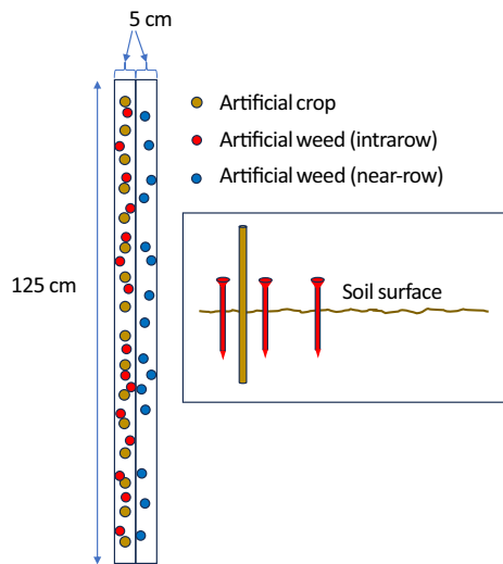
Figure 2. Quadrat dimensions and installation of artificial crop and weeds in soil bin studies. The long narrow quadrats were intended to improve resolution of efficacy measurements of the finger weeder. Artificial weeds were randomly sown in the intra- and near-row zones, using unique colors to track responses in each.
