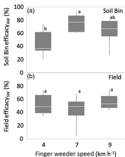
Figure 8. Finger weeder speed effects on efficacy using artificial weeds (Efficacy AW ) in the soil bin (A) and using a surrogate weed (Efficacy SW ; Brassica juncea ) in 2021 and 2022 field experiments. Treatments with common letters are not statistically different using Tukey's Honestly Significant Difference at \alpha \leq 0.05 . Box plots show median center lines, upper and lower quartiles, with whiskers at 1.5 \times the interquartile.
