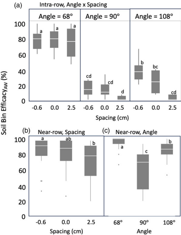
Figure 6. Finger weeder angle and spacing effects on efficacy using artificial weeds (AWs, 70-mm-long wooden golf tees) in a soil bin showing the interaction of angle \times spacing on AWs in the intrarow (A), and the main effect of spacing (B) and angle (C) on AWs in the near-row zone. Treatments with common letters are not statistically different using Tukey's Honestly Significant Difference at \alpha \leq 0.05 . Box plots show median center lines, upper and lower quartiles, with whiskers at 1.5 \times the interquartile; outliers are also shown.
