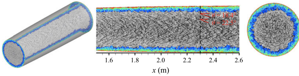
Figure 26. Numerical schlieren images (i.e. density gradient contours) of radiated acoustic waves within the nozzle of the Sandia HWT-8 (Duan et al. 2019b). The vertical dashed line indicates the axial location of the selected cross-section visualised in the right panel.
