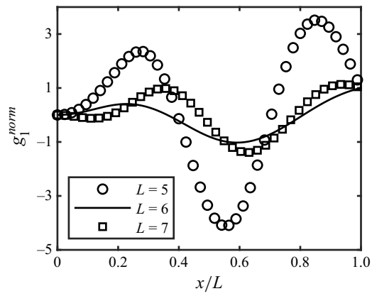
Figure 29. Normalized profiles of u'_x of the linear perturbation mode m = 1 for three different pipe lengths.
