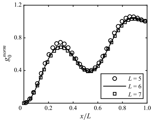
Figure 28. Normalized profiles of u'_x at the central axis of the linear perturbation mode m = 0 for three different pipe lengths.
