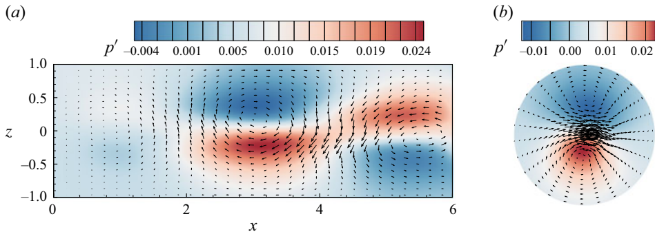
Figure 32. Planar projected perturbation velocity vectors and contours of perturbation pressure for the case Re = 700 and \omega = 4.3 at t = 2 (time-dependent inlet velocity profile): (a) x - z plane; (b) \theta - r plane at x = 3 .
