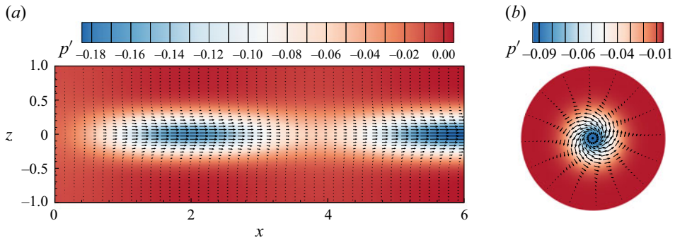
Figure 3. Projected perturbation velocity vectors and contours of perturbation pressure for the case Re = 5000 and \omega = 3.85 at t = 6000 : (a) in the x - z plane, (b) in the \theta - r plane at x = 3 .
