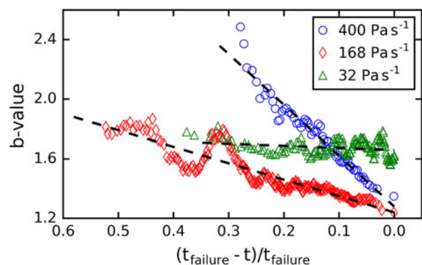
Fig. 9. Evolution of b -value before complete failure for different loading rates (400, 168 and 32 \text{Pa s}^{-1} ). The dashed lines represent a linear regression. Samples shown: LDL07A, LDL12B and LDL04B_load02, window size n = 250 .
