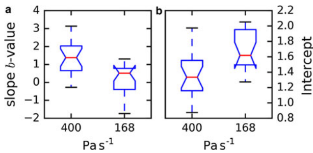
Fig. 10. Boxplots summarizing the linear regression to the b -value time evolution of several samples for two different loading rates (168 Pa s -1 , N = 18 ; 400 Pa s -1 , N = 19 ). (a) The slope of the b -value evolution with time. (b) b -value at failure obtained from the intercept of the linear fit at the failure point.
