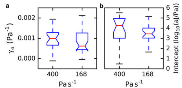
Fig. 12. Boxplots summarizing the temporal evolution of the energy rate for several samples and for two different loading rates (168 Pa s -1 , N = 18 ; 400 Pa s -1 , N = 19 ). (a) Exponential coefficient \gamma_{\sigma} . (b) Energy rate at failure (logarithmic scale) obtained from the intercept of the linear fit at the failure point.
