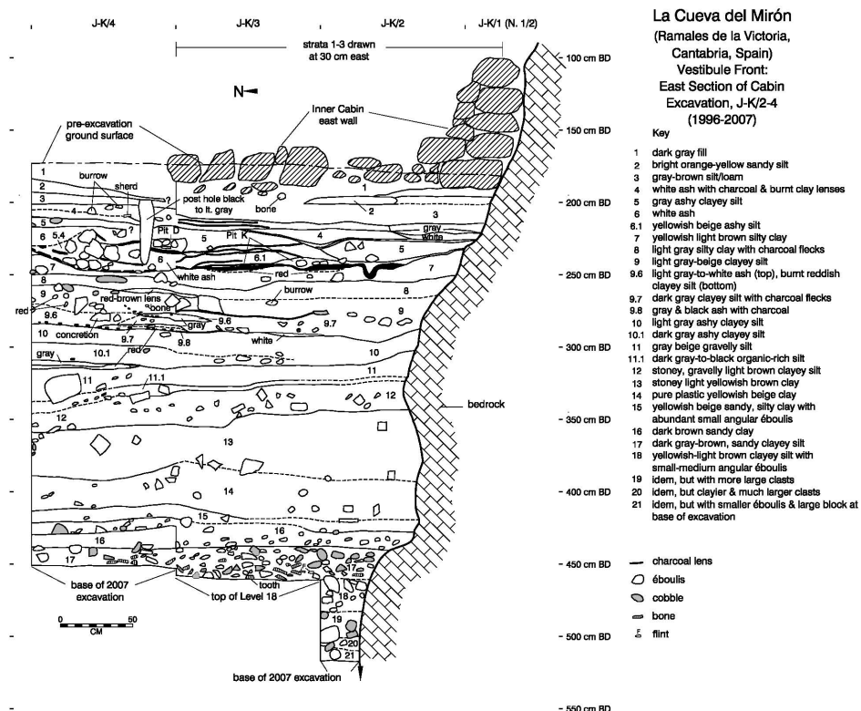
Figure 1 Stratigraphy of El Mirón Cave
