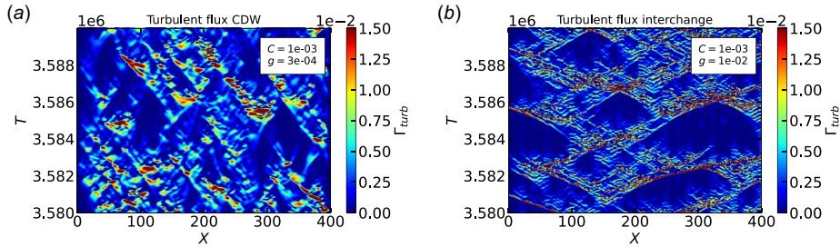
FIGURE 12. Examples of turbulent flux of particles \Gamma_{turb} = -2k_y \mathfrak{S}(N_k \phi_k^*) at steady state. (a) (C, g) = (10^{-3}, 3 \times 10^{-4}) . (b) (C, g) = (10^{-3}, 10^{-2}) . Both are computed with a fixed source at S_N(0) = 10^{-4} .
