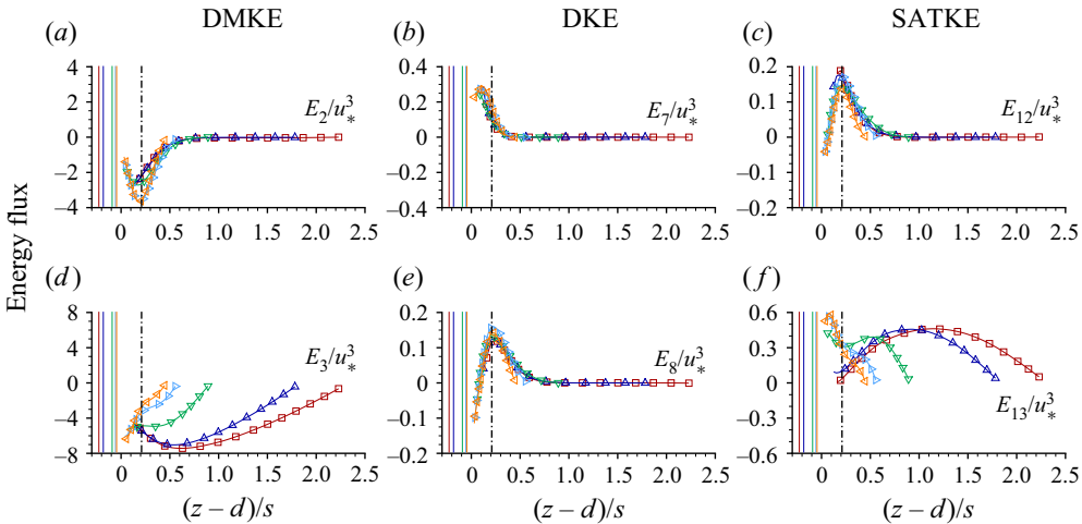
Figure 13. Distributions of energy fluxes as functions of (z-d)/s : (a) E_2 = \phi\langle\bar{u}_i\rangle\langle\bar{u}_i\bar{w}\rangle ; (b) E_7 = \phi\langle\bar{u}_i\bar{u}_i\bar{w}\rangle ; (c) E_{12} = \phi\langle\bar{u}_i\bar{u}_i\bar{w}\rangle ; (d) E_3 = \phi\langle\bar{u}_i\rangle\langle\bar{u}_i\bar{w}'\rangle ; (e) E_8 = \phi\langle\bar{u}_i\bar{u}_i\bar{w}'\rangle ; (f) E_{13} = \phi\langle\bar{u}_i\bar{u}_i\bar{w}'\rangle . Symbols and vertical lines are defined in figure 4.
